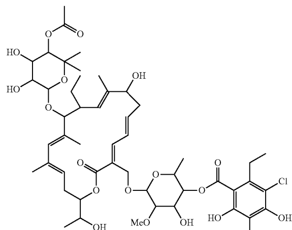
Compound 101
