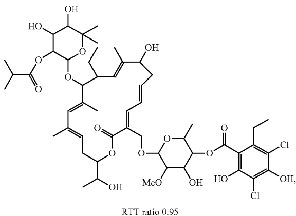
Compound 111
