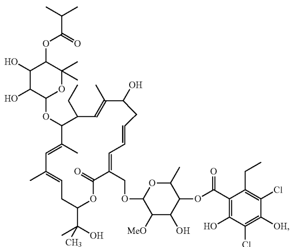
Compound 105
