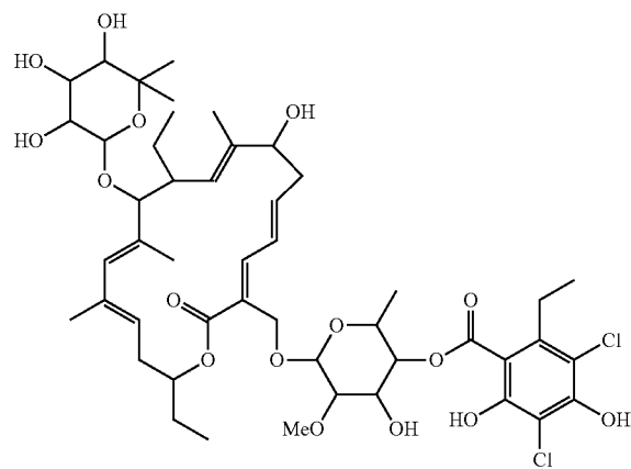
Compound 102
