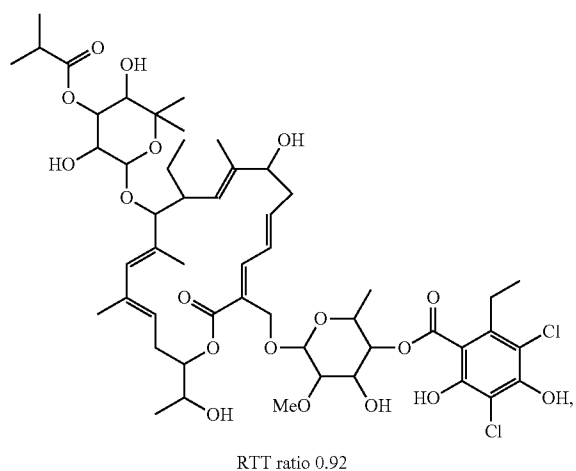
Compound 111
