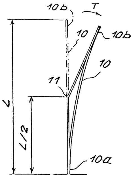
FIG. 1 PRIOR ART
