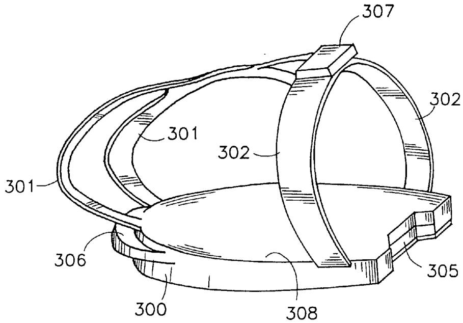
FIG. 11 (PRIOR ART)
