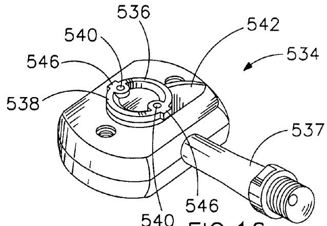
FIG. 16 (PRIOR ART)
