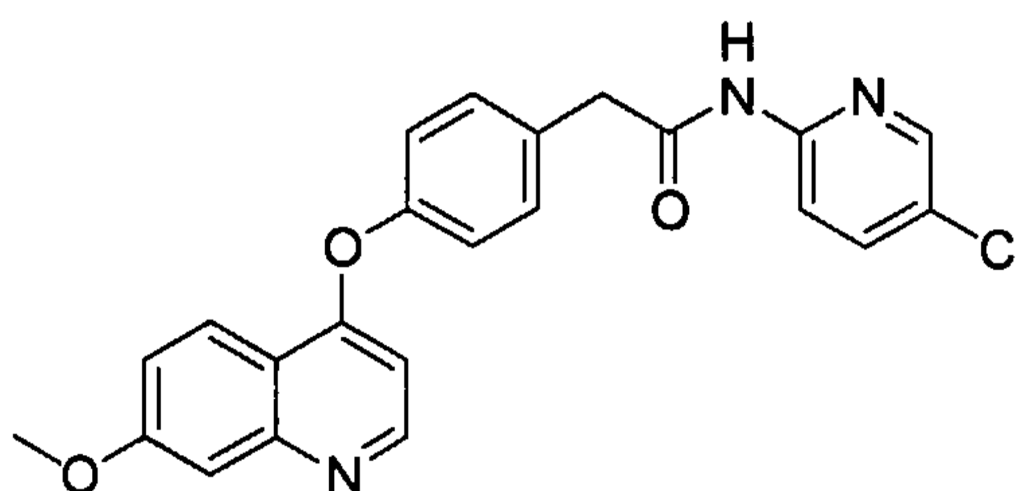
Intermediate 4-chloro-7-methoxy-quinoline
