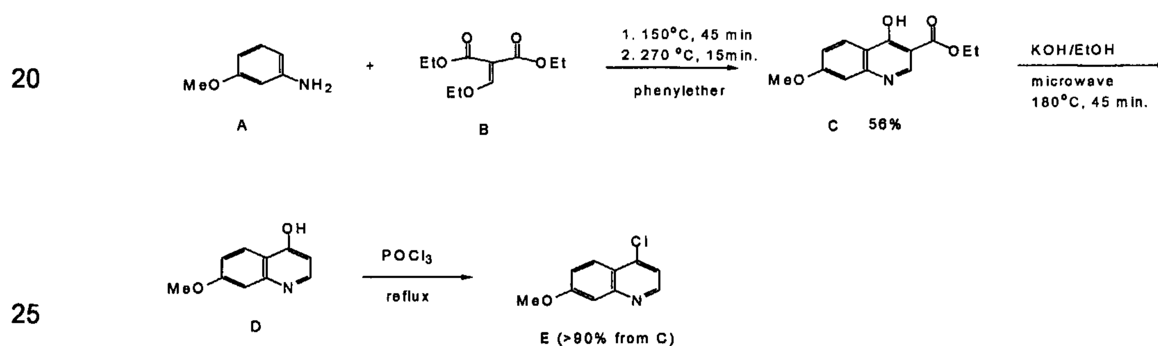
Intermediate 4-chloro-7-methoxy-quinoline
