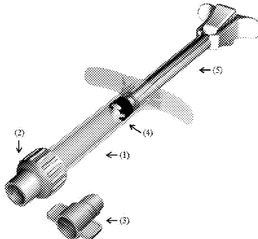
Medmix syringe mixing system
