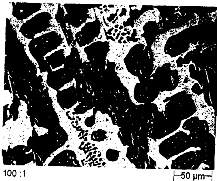
Ledeburite with martensite (Ni Hard 1)
