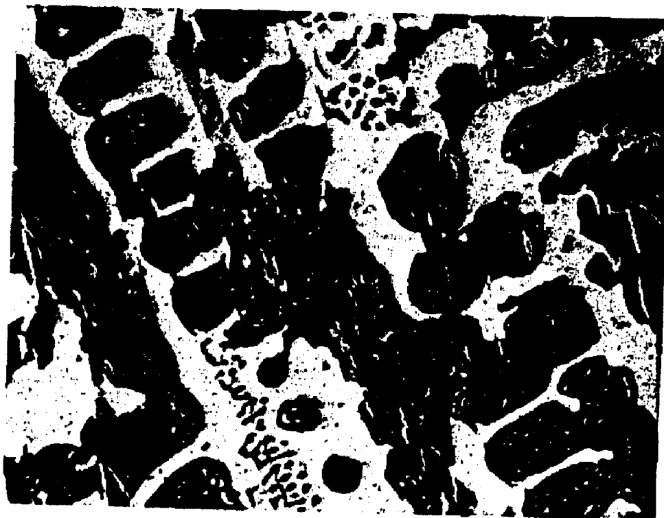
Ledeburite with martensite (Ni Hard 1)
