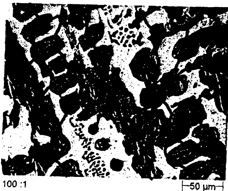
Objective: Ledeburite with martensite and graphite flakes (schematic)
