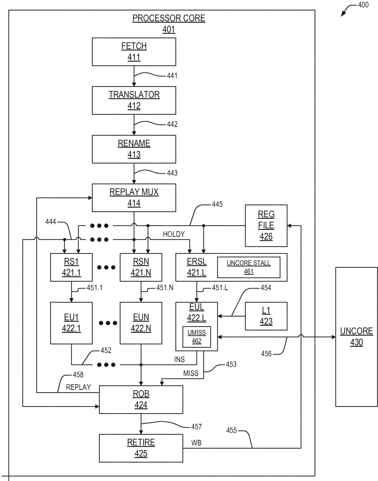
EXEMPLARY CORE STAGES FOR LOAD REPLAY REDUCTION
