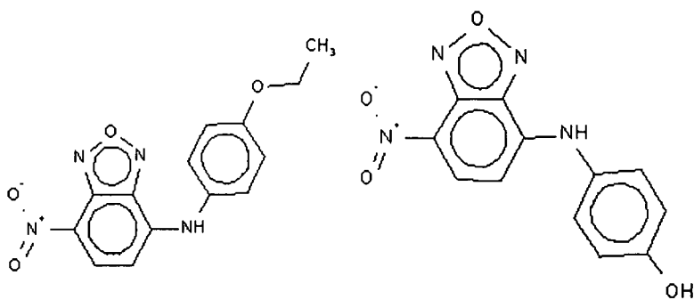
Compound 146
