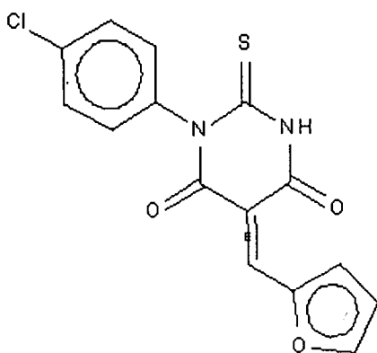
Compound 261
