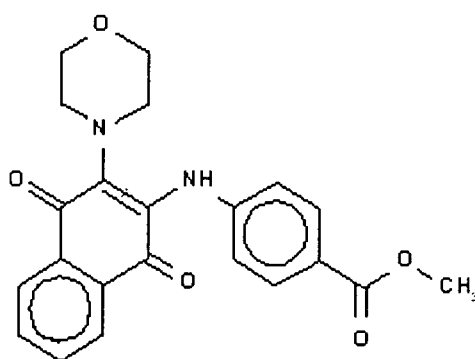
Compound 142
