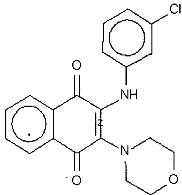
Compound 133
