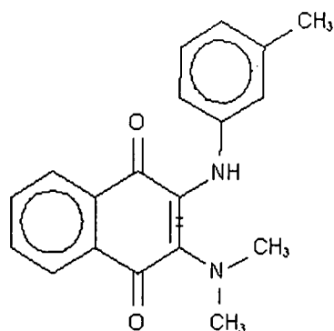
Compound 204
