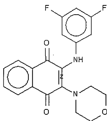
Compound 204
