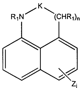
Formula P
