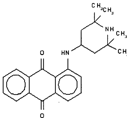
Compound 110
