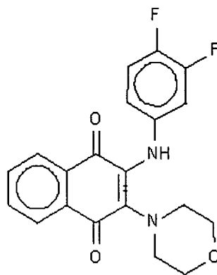
Compound 187
