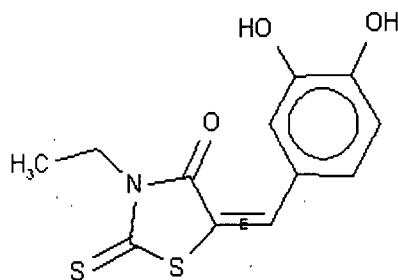
Compound 365
