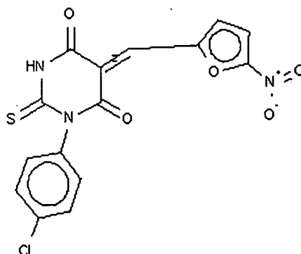
Compound 257
