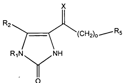
Formula R
