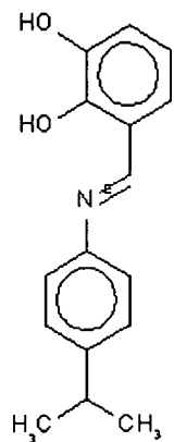
Compound 9
