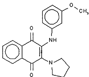
Compound 104
