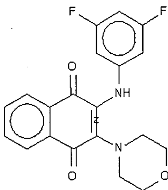
Compound 204
