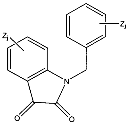
Formula L
