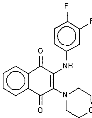
Compound 187
