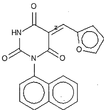
Compound 137
