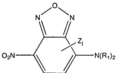
Formula D-A
