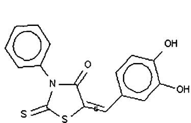
Compound 292
