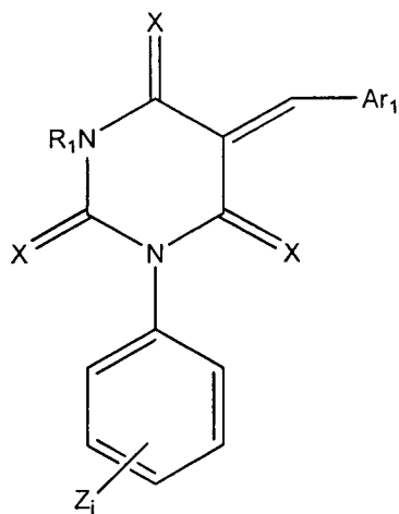
Formula S
