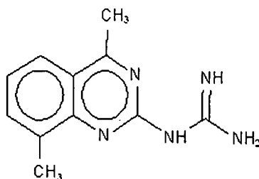
Compound 349
