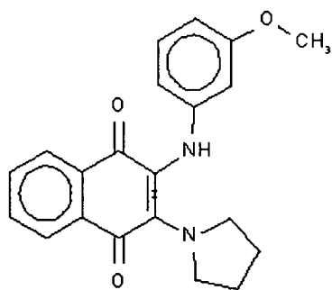
Compound 104
