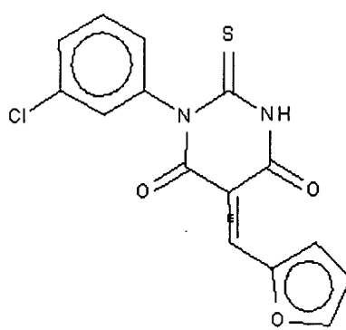
Compound 322
