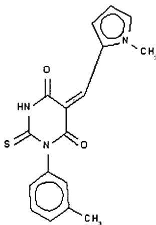
Compound 149
