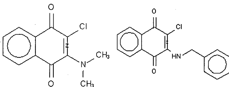
Compound 174
