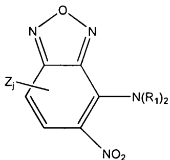
Formula D
