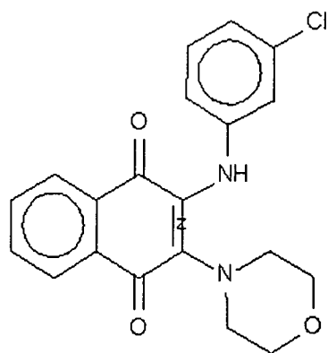
Compound 133
