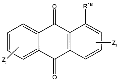
Formula H-B
