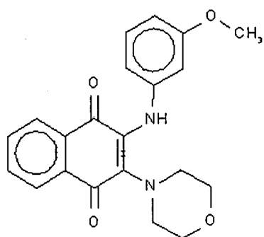
Compound 120
