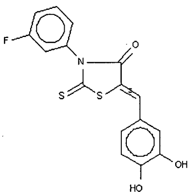
Compound 292
