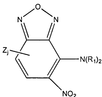
Formula D
