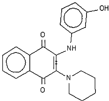
Compound 152
