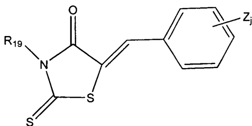
Formula V
