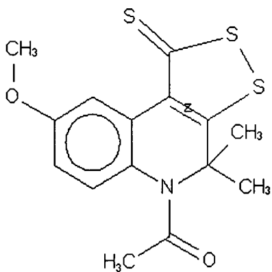
Compound 238
