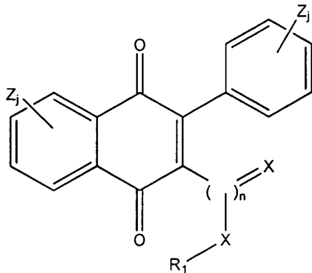
Formula G
