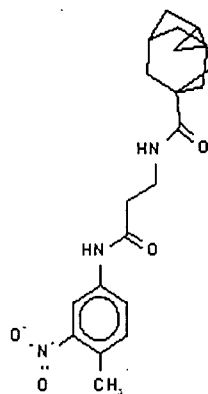
Compound 13
