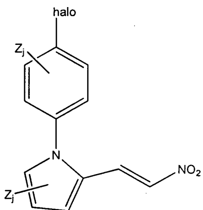
Formula E
