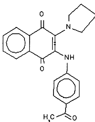
Compound 130
