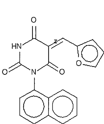
Compound 137
