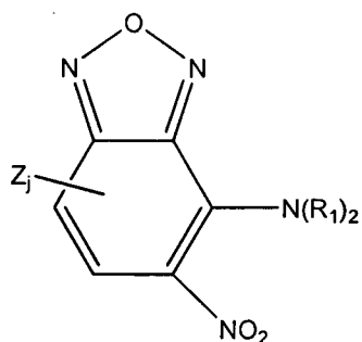
Formula D
