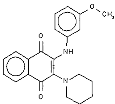
Compound 95
