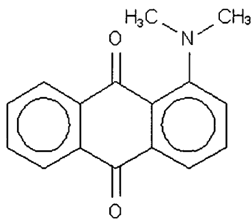
Compound 121
