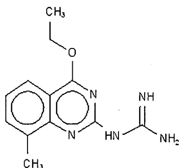
Compound 122
