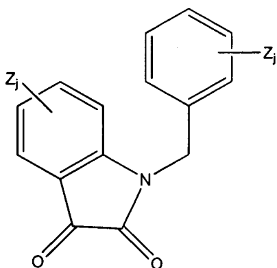
Formula L
