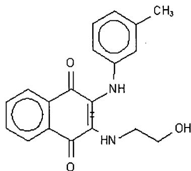
Compound 215
