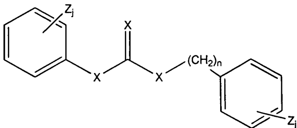
Formula N-I
