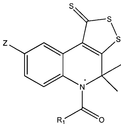
Formula U-1
