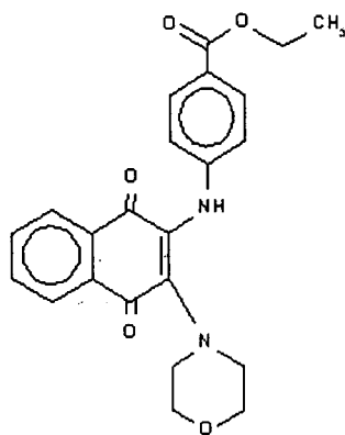
Compound 119
