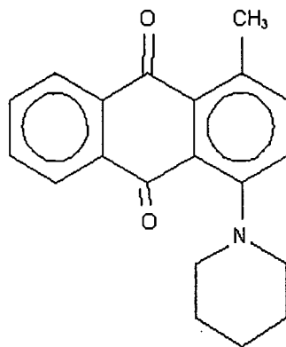
Compound 110
