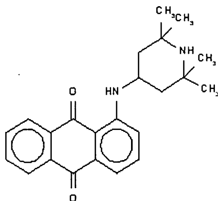
Compound 178
