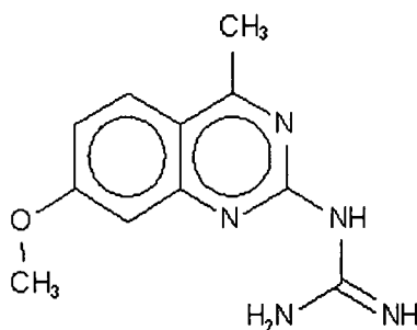
Compound 188
