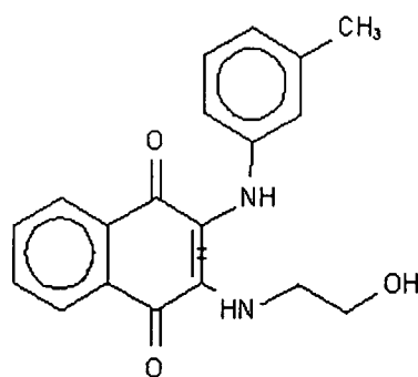
Compound 215
