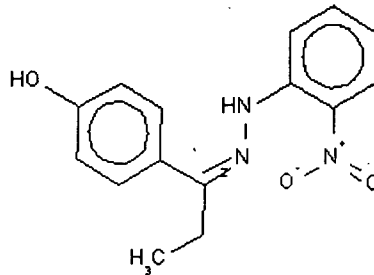
Compound 186
