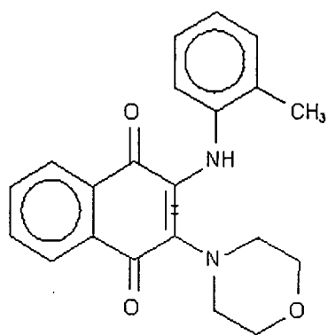
Compound 118
