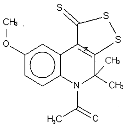
Compound 238
