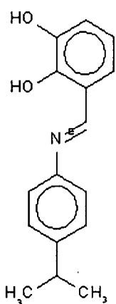
Compound 9
