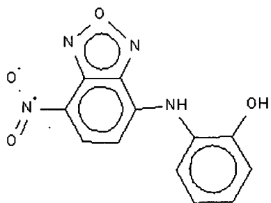
Compound 210
