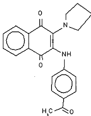
Compound 130
