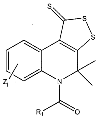
Formula U
