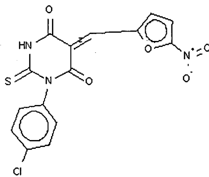
Compound 257
