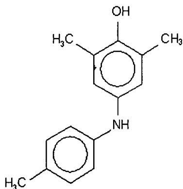
Compound 193
