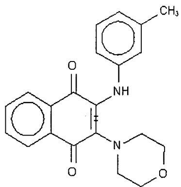
Compound 107
