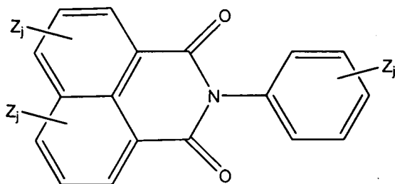
Formula O
