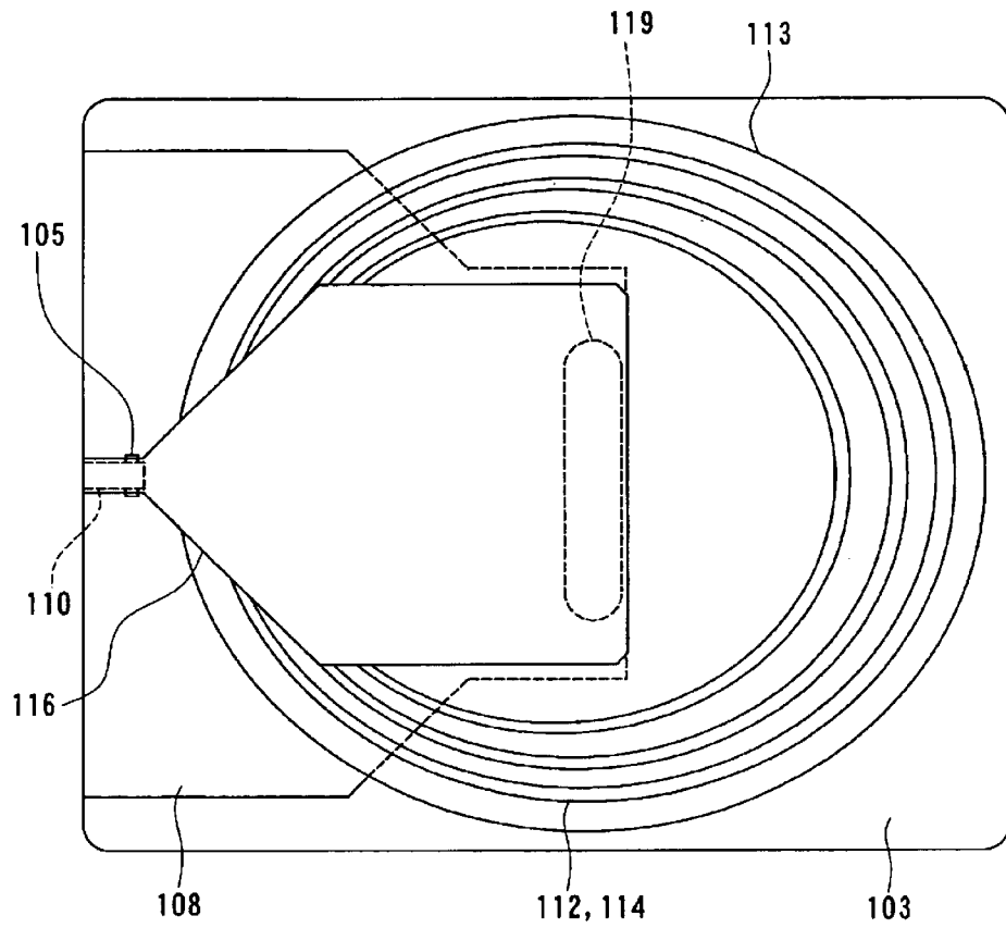
FIG. 36 RELATED ART
