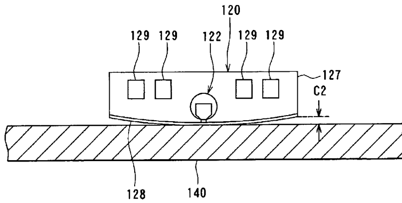
FIG. 40 RELATED ART
