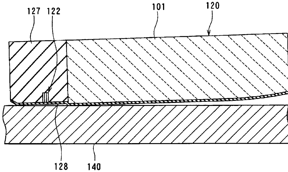
FIG. 41 RELATED ART
