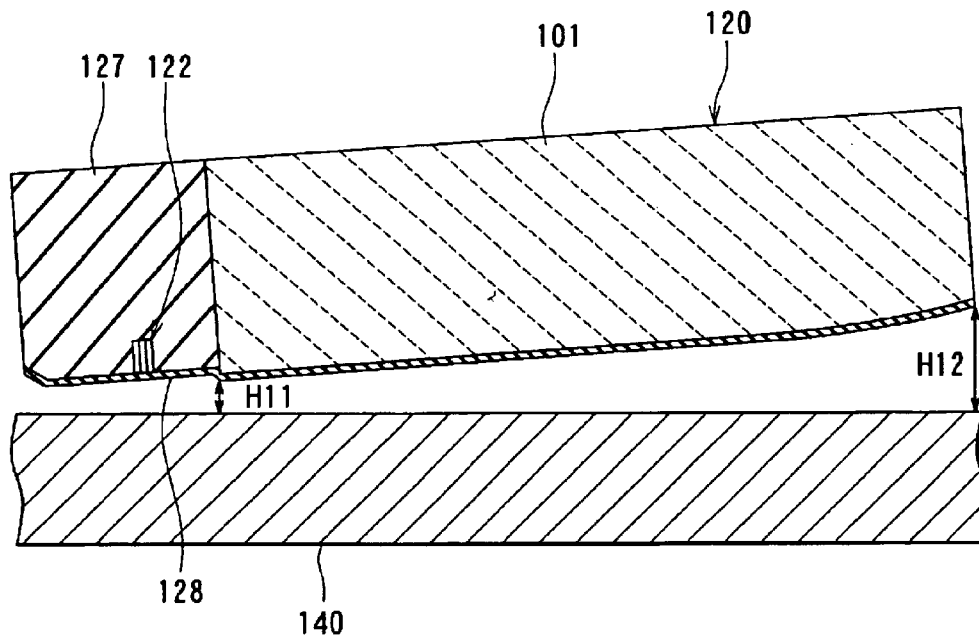
FIG. 42 RELATED ART
