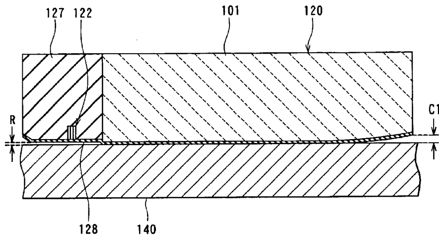
FIG. 39 RELATED ART
