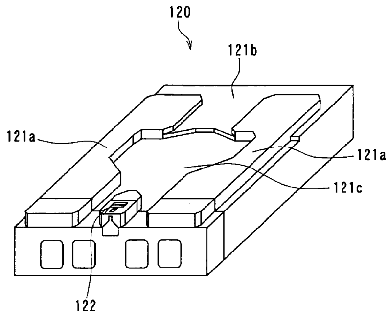
FIG. 38 RELATED ART
