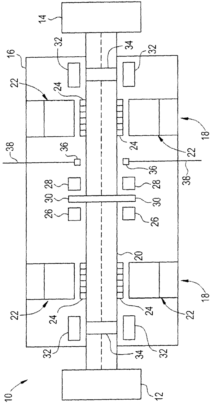
FIG. 1 PRIOR ART
