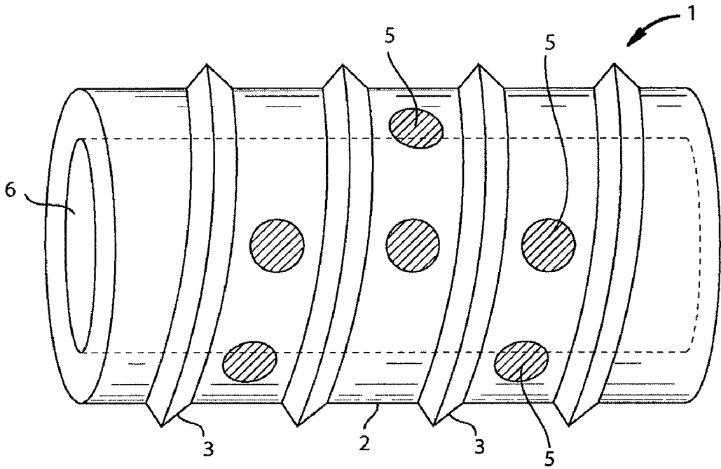
FIG. 13 (PRIOR ART)
