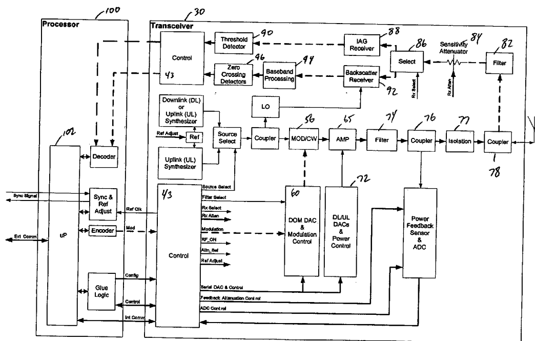
Figure 10 Built-In-Test Loop-Back Path
