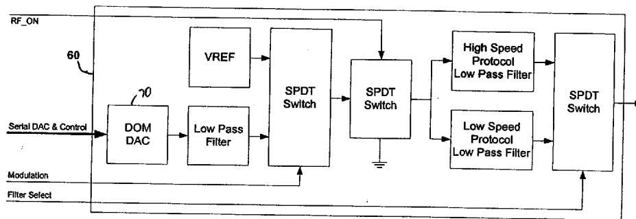
Figure 7 DOM DAC and Modulation Control Block Diagram
