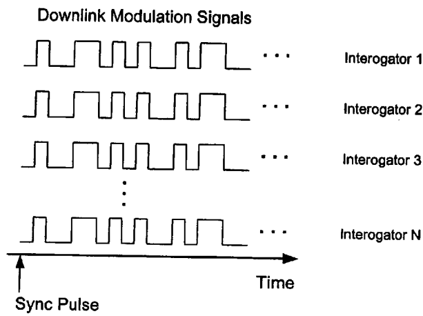
Figure 3(b) - Step Lock with Bit Synchronization
