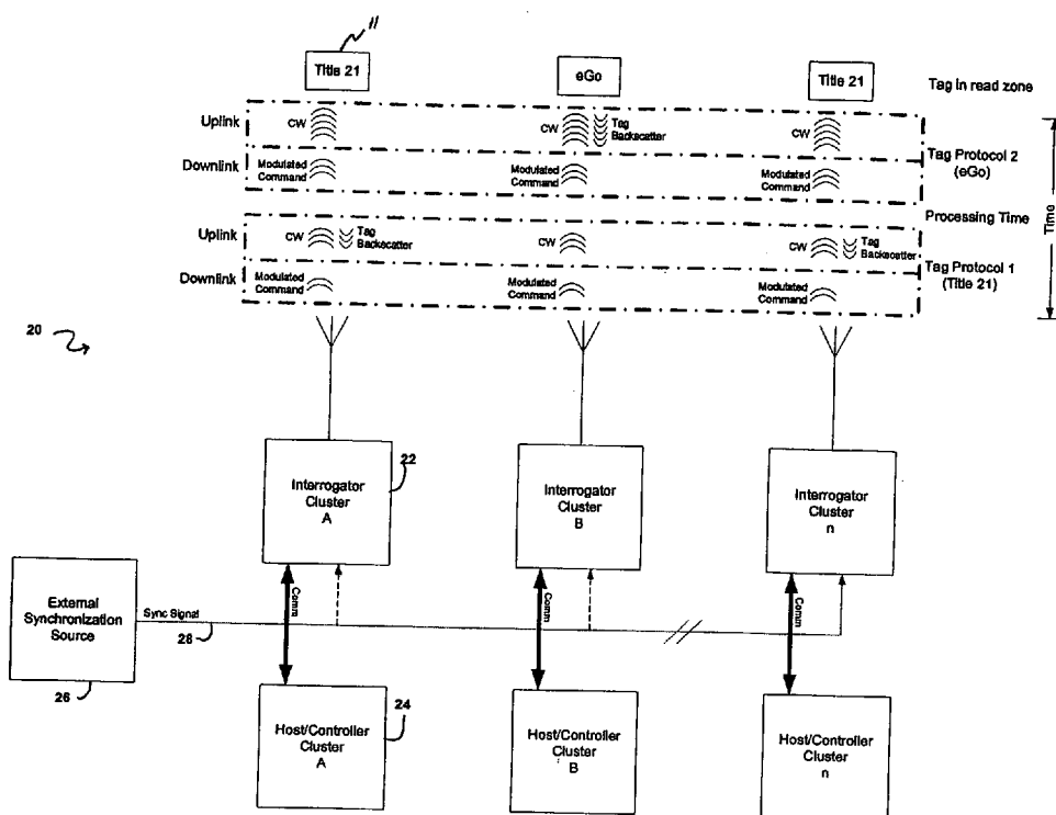
Figure 2 Step-Locked Interrogator Clusters (External Sync Signal)
