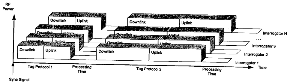
Figure 3(a) - Step Lock Timing Diagram
