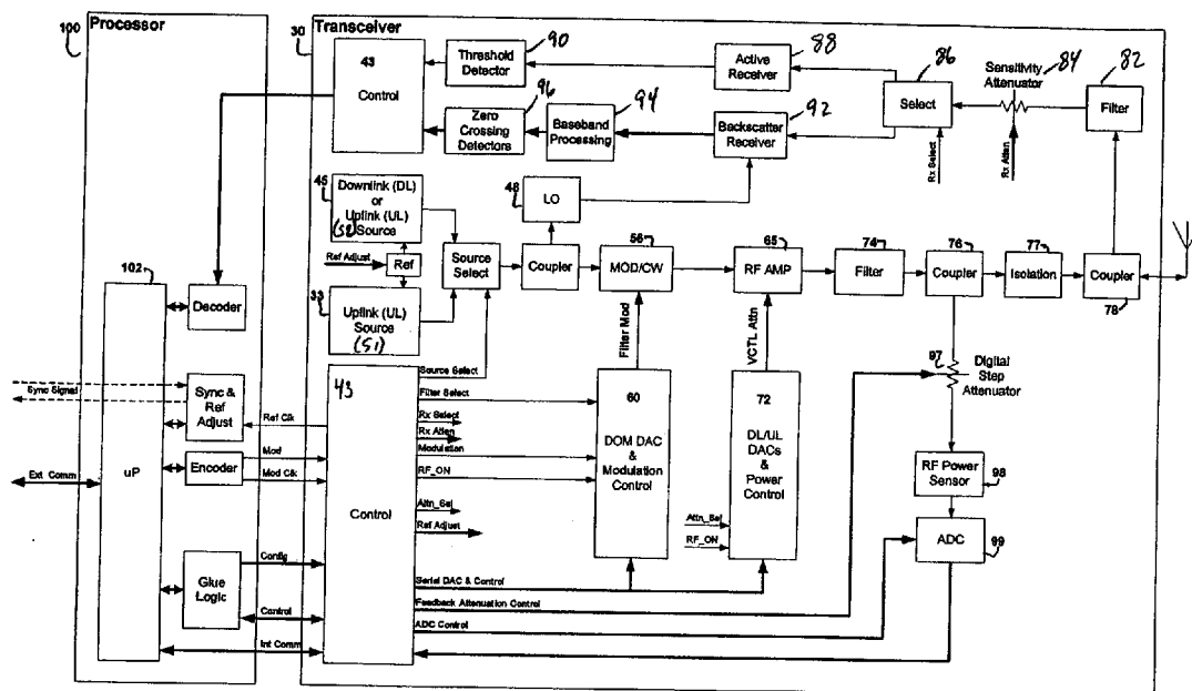
Figure 4 Interrogator Block Diagram
