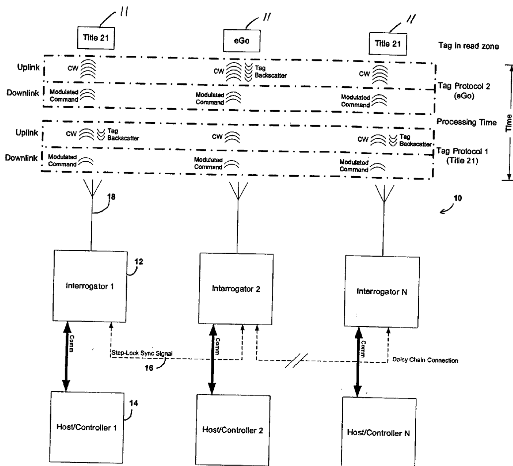
Figure 1 Step-Locked Interrogator Cluster (Internal Sync Signal)
