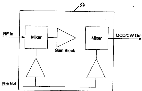
Figure 6 Dual Mixer Block Diagram
