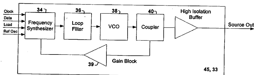
Figure 5 Synthesized Source Block Diagram
