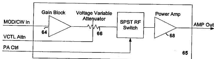
Figure 8 Power Amplifier Block Diagram
