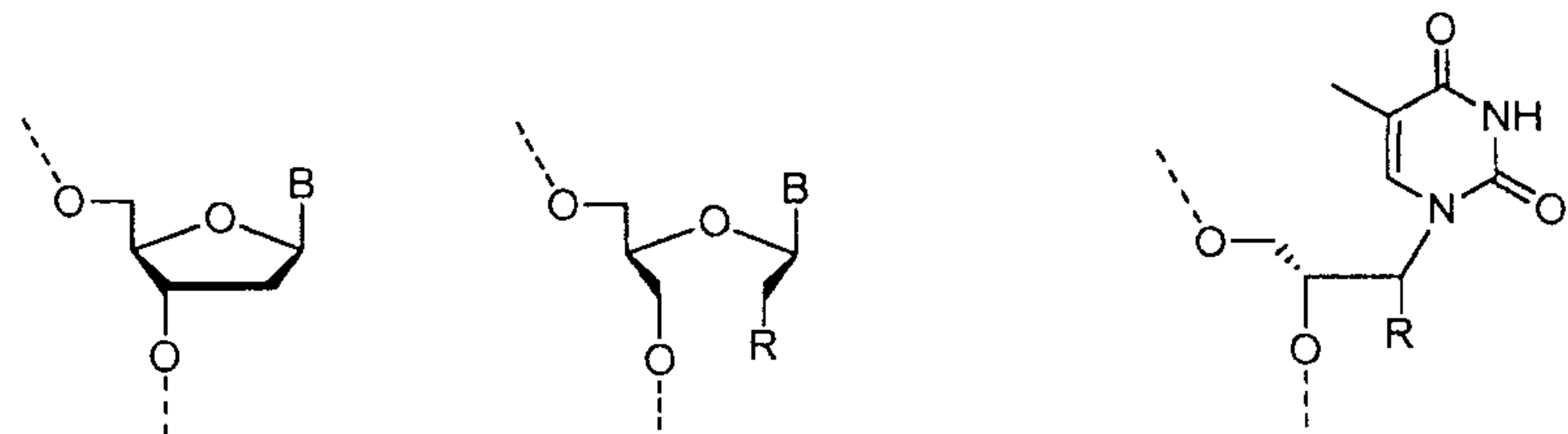
unlocked nucleic acid R= H, OH, O-alkyl
