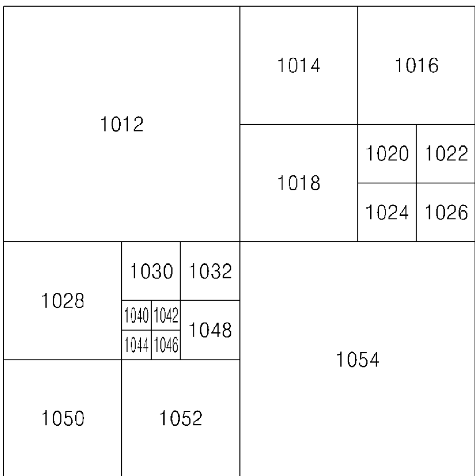
CODING UNITS (1010)
