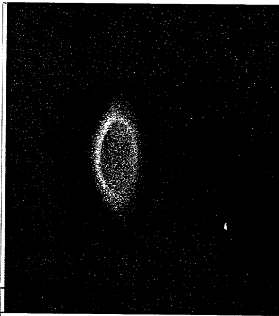
Near-Field Mirror Illumination Pattern
