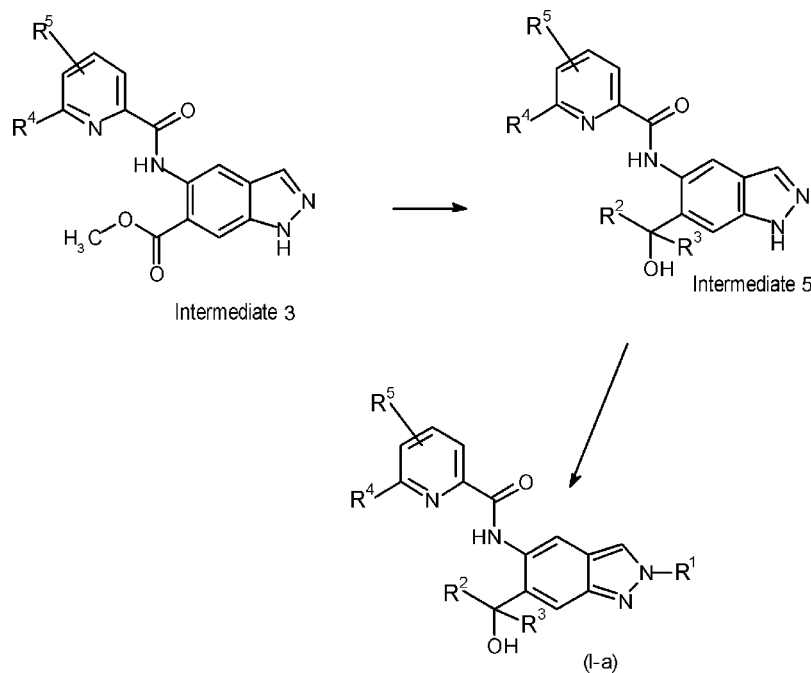
Synthesis Scheme 4
