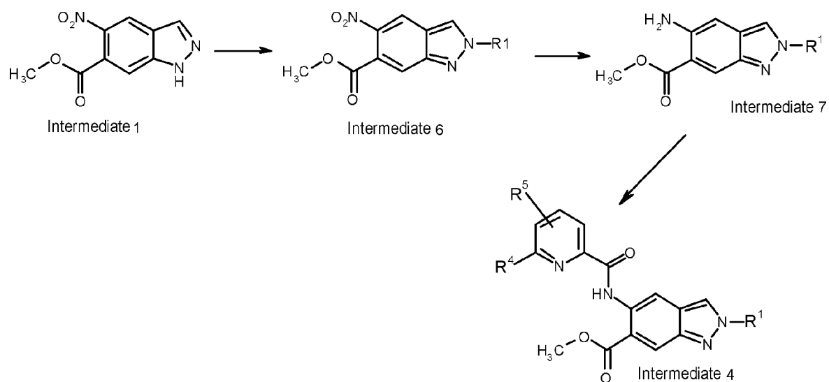
Synthesis Scheme 5
