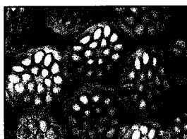
18 Island-in-Sea, 50/50% Nylon/PE
