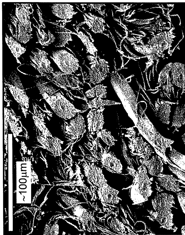
1 Hydro Pass + Point Bonded at 145 °C 100 - 120 gsm
