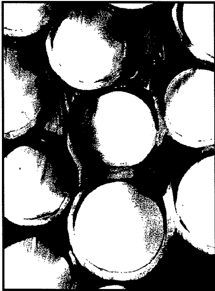
Sheath-Core (1 Island-in-Sea), 75/25% Nylon/PE
