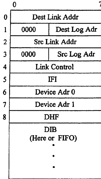
Device Frame Header Structure
