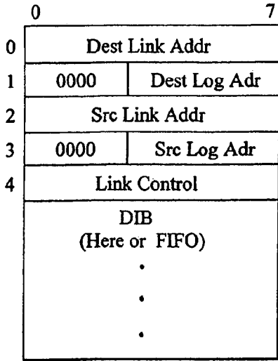
Link Frame Header Structure.
