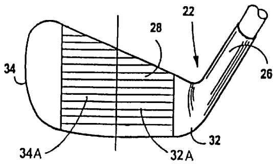
FIG 6 (PRIOR ART)
