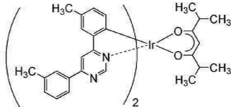
[Ir(5mdppm) 2 (dibm)]
