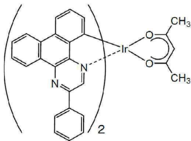
[0228] [Ir(dbq-P) 2 (acac)]
