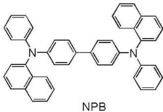
NPB
