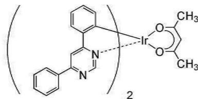
[Ir(dppm)_2(acac)]
