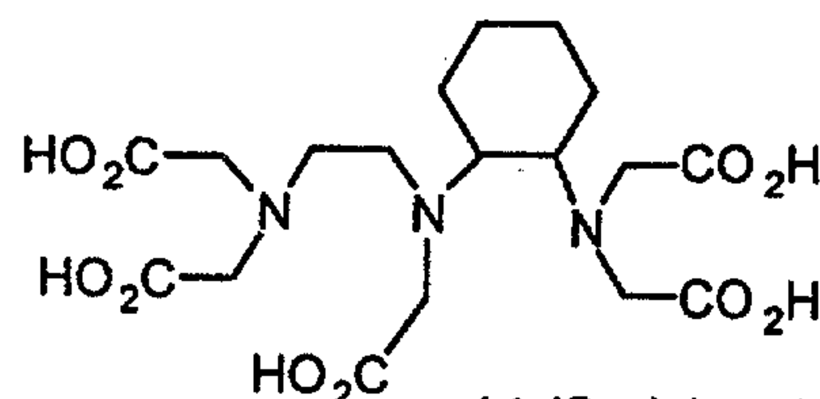
14 (Cyclohexyl-DTPA)
