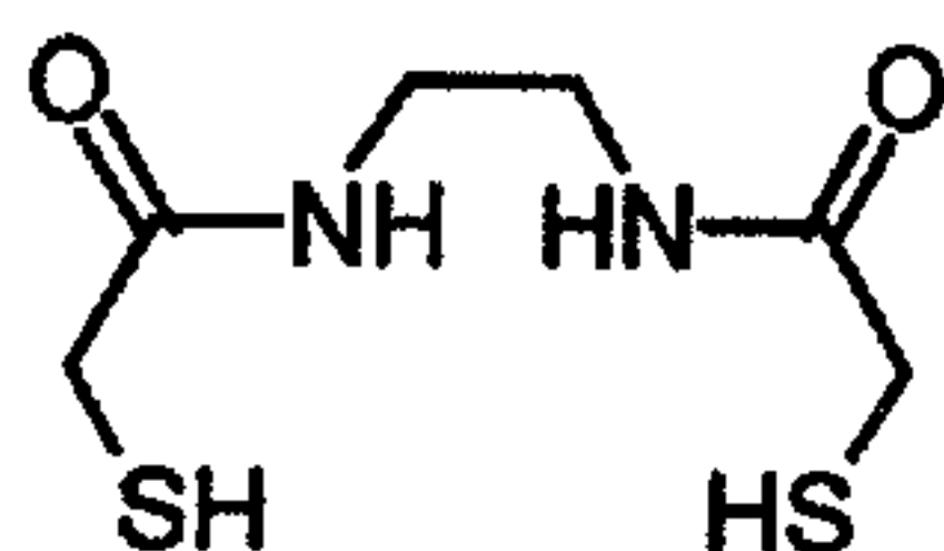
9 (N 2 S 2 )
