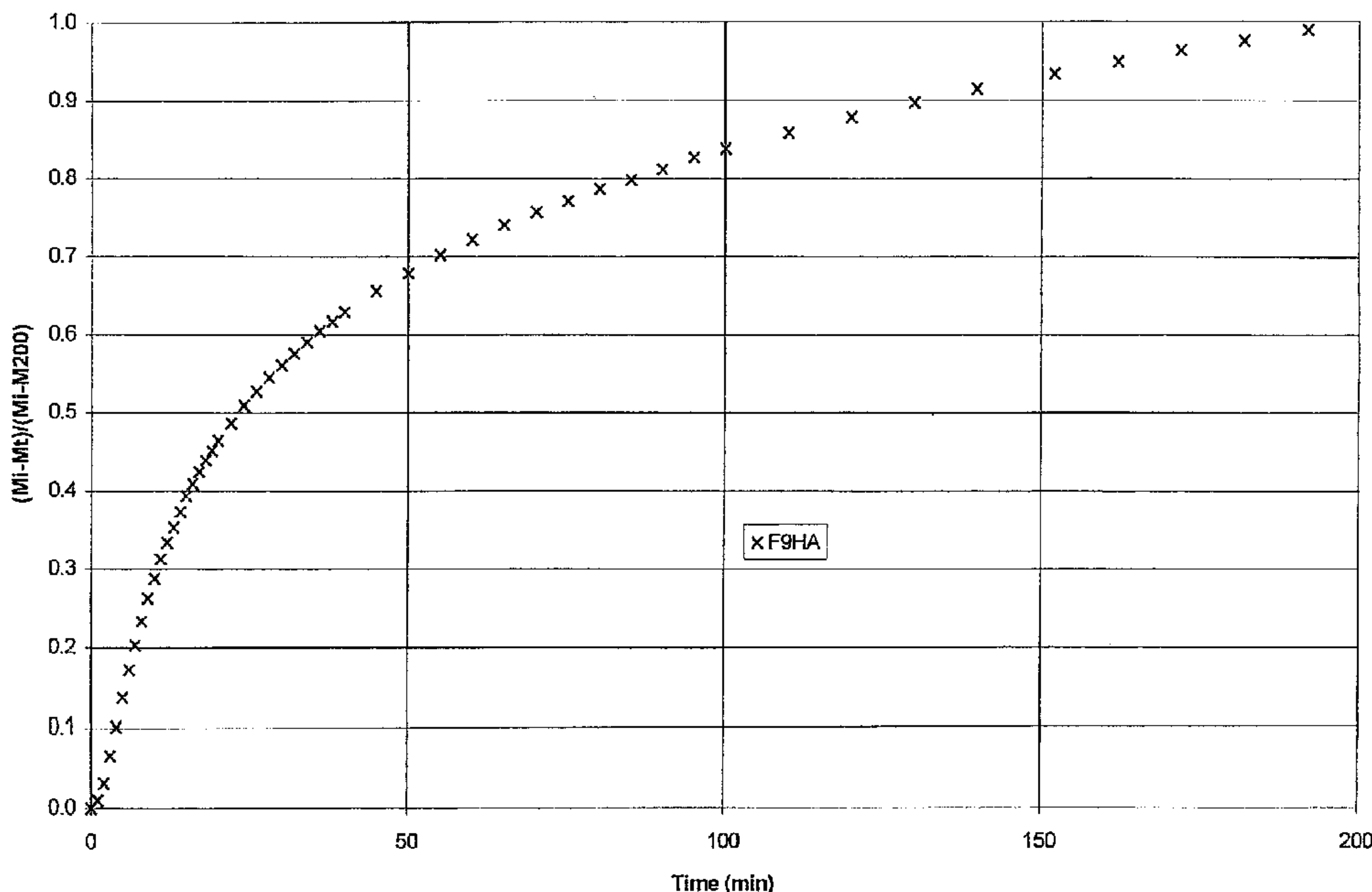
NaX Water Desorption Curve
