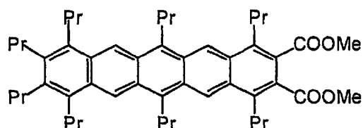
Dimethyl 1,4,6,8,9,10,11,13-octapropylpentacene-2,3-dicarboxylate
