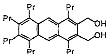
2,3-Bis(hydroxymethyl)-1,4,5,6,7,8-hexapropylantracene:
