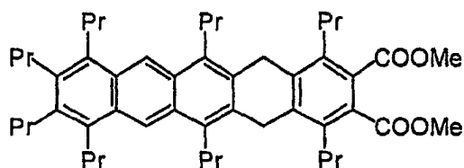
Dimethyl 5,14-dihydro-1,4,6,8,9,10,11,13-octapropylpentacene-2,3-dicarboxylate
