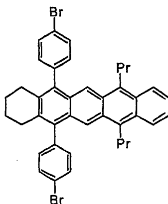
5,14-Bis(p-bromophenyl)-7,12-dipropyl-1,2,3,4-tetrahydropentacene
