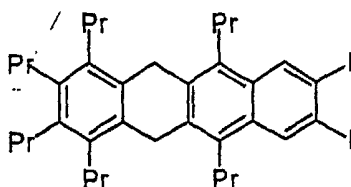
6,11-Dihydro-2,3-diiodo-5,7,8,9,10,12-hexapropylnaphthacene
