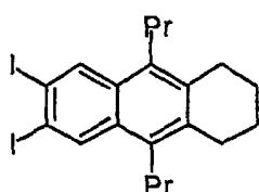
9,10-Dipropyl-2,3-diiodo-5,6,7,8-tetrahydroanthracene
