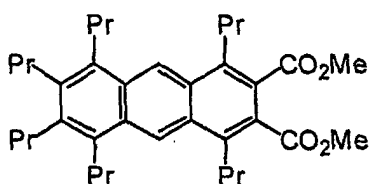
Dimethyl 1,4,5,6,7,8-hexapropylantracene-2,3-dicarboxylate
