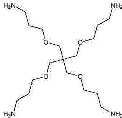
3-[3-(3-amino propoxy)-2,2-bis(3-amino-propoxymethyl)-propoxy]-propylamine, or 4 AA
