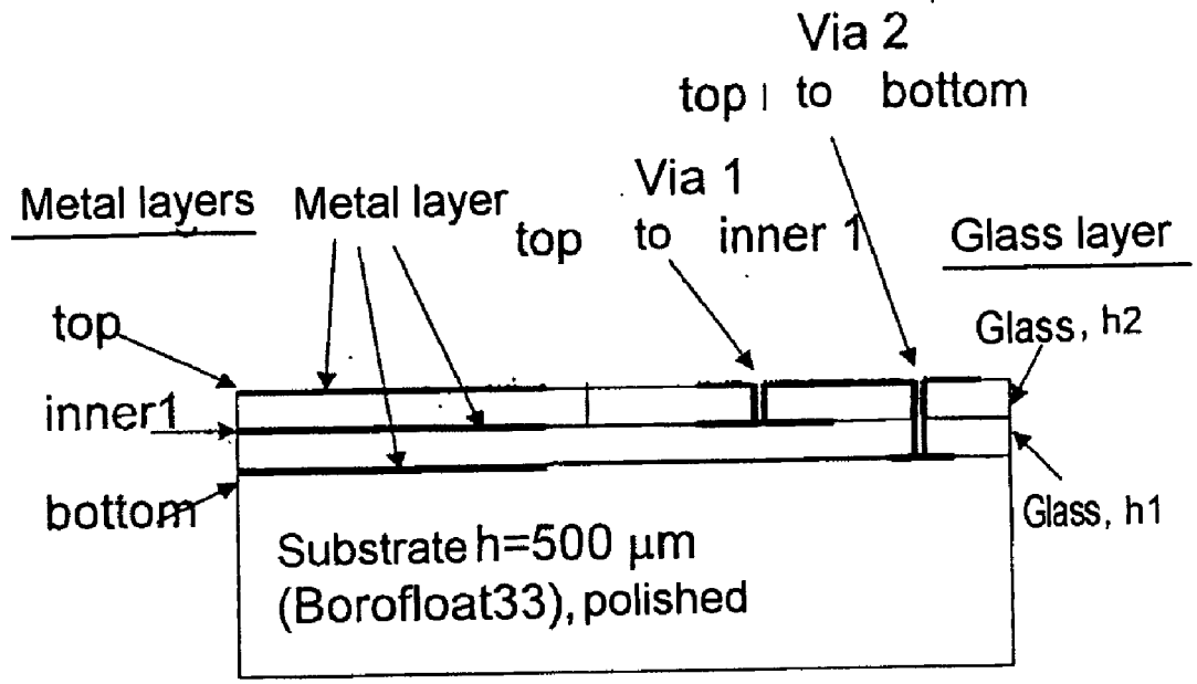
Fig. 8 Diagrammatic layer arrangement for RF measurement
