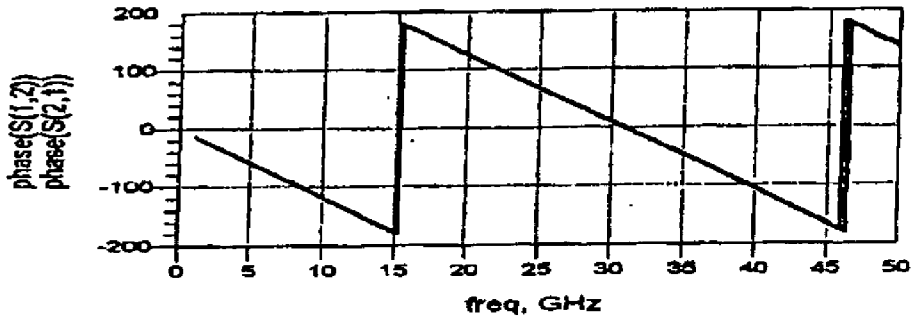
Fig. 23: Phase profile S21 for specimen G2ACPW3_2
