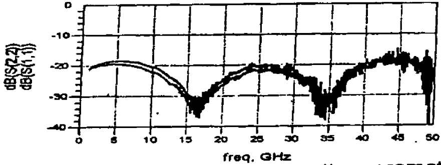
Fig. 12: Magnitude of the scatter parameter S11 for specimen G1ACPW2_2
