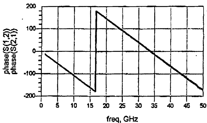
Fig. 20: Phase profile S21 for specimen G2ACPW2_6
