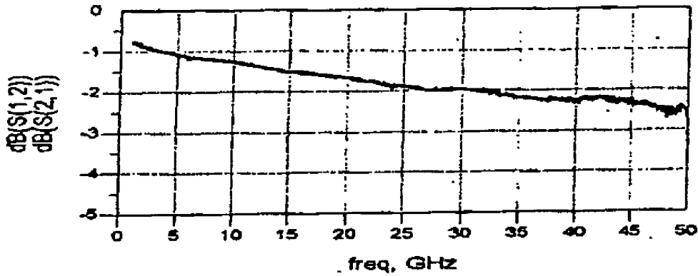
Fig. 16: Magnitude of the scatter parameter S21 for specimen G1ACPW3_2
