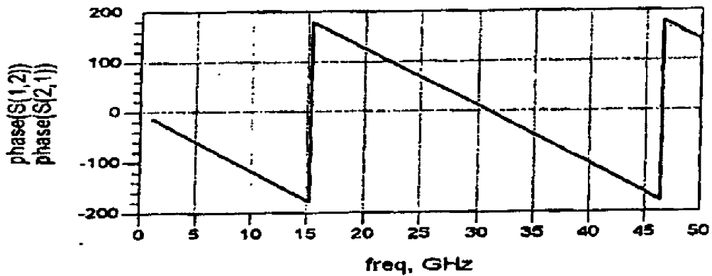
Fig. 17: Phase profile S21 for specimen G1ACPW3_2
