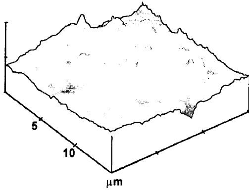
Titanium
