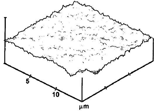
Titanium + FSNP
