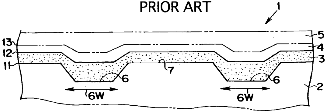
Fig.17 PRIOR ART
