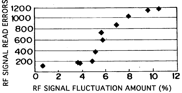
Fig.21 PRIOR ART
