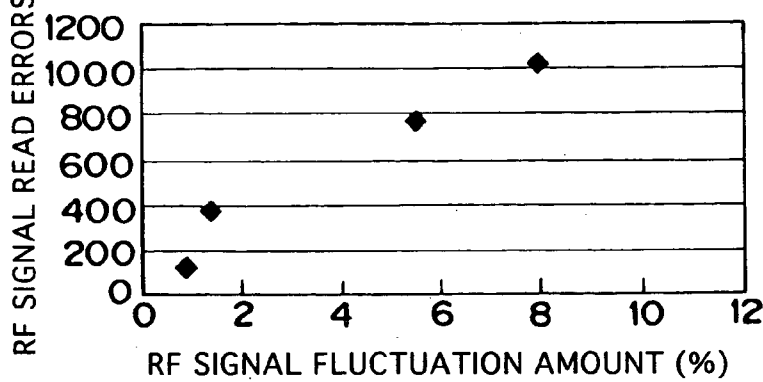
Fig.22 PRIOR ART
