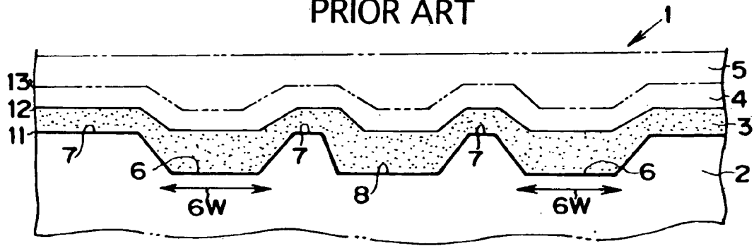
Fig.18 PRIOR ART
