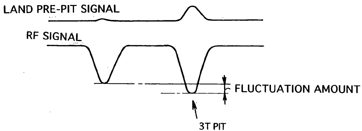
Fig.24 PRIOR ART
