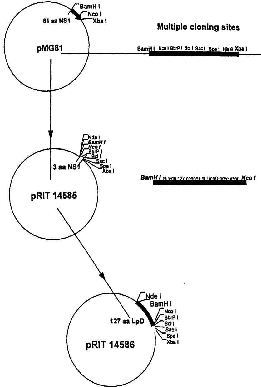
FIGURE 2 : Construction of the expression vector pRIT 14586
