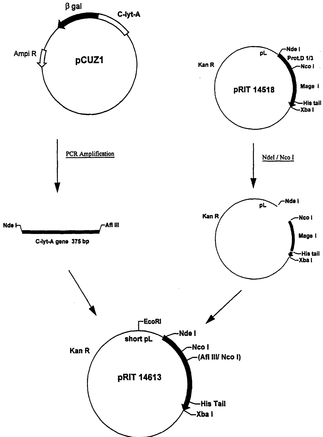
Figure 16 : construction of plasmid pRIT 14613.
