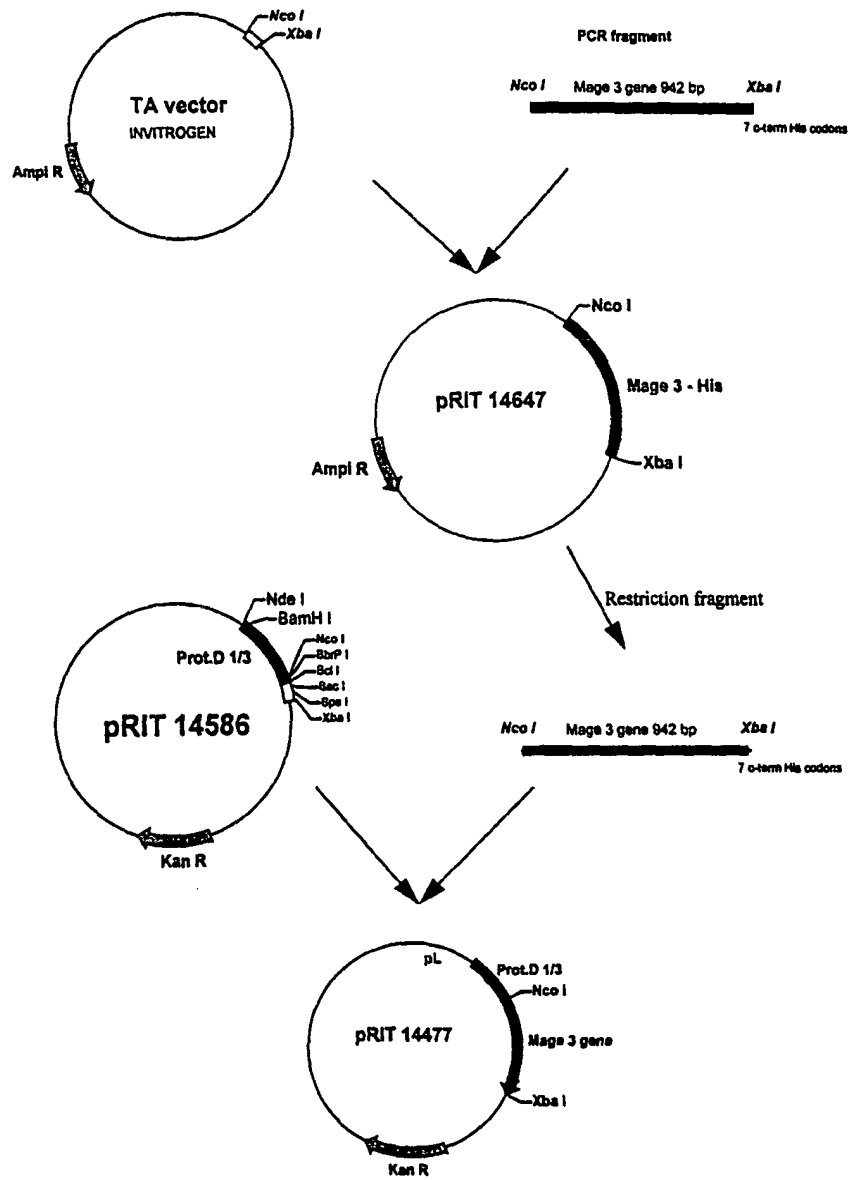
FIGURE 3 : Construction of plasmid pRIT 14477 expressing the fusion protein Prot. D 1/3-MAGE-3-His tail
