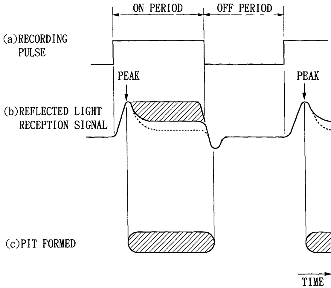
FIG. 4 PRIOR ART
