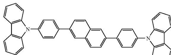
(H-3)
