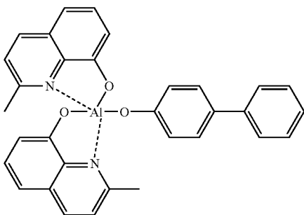
BAQ
