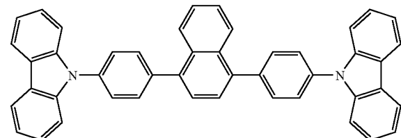
(H-3)
