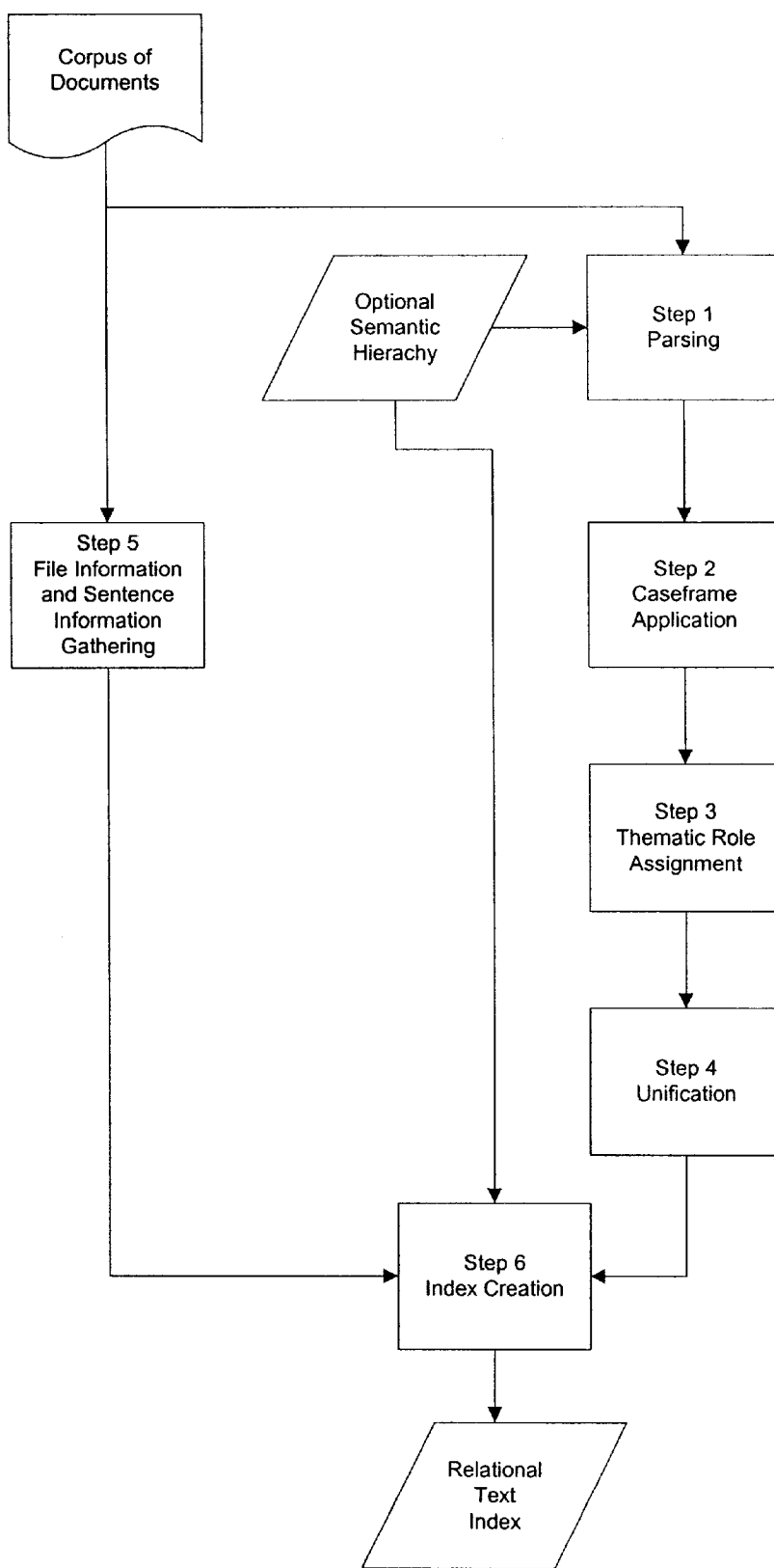
Figure 3 Index Creation Algorithm, High Level
