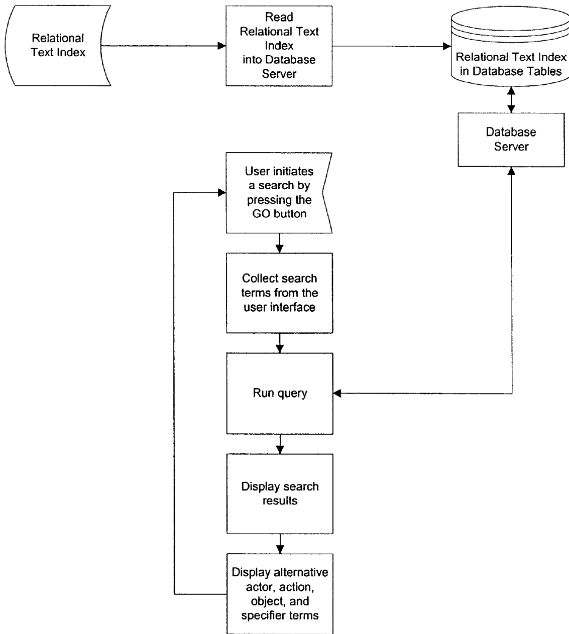
Figure 6 Flowchart – PowerDrill
