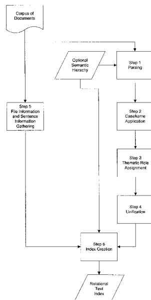
Index Creation Algorithm, High Level
