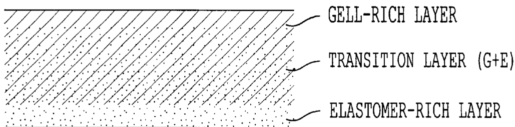
FIG. 1B PRODUCT OF THE PRESENT INVENTION
