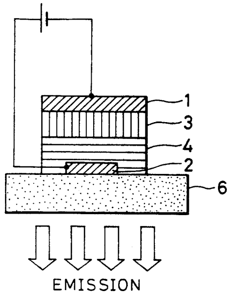
FIG. 1 (PRIOR ART)
