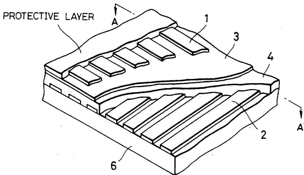
FIG. 3 (PRIOR ART)
