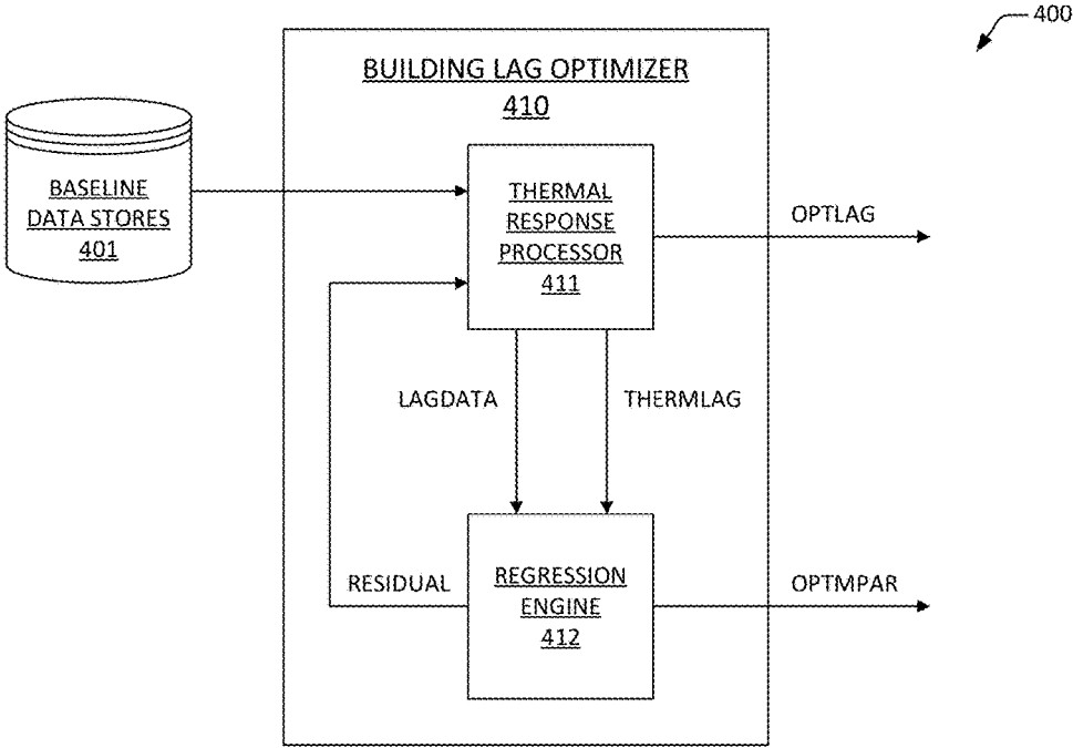
FIG. 4 FINE-GRAINED BASELINE ENERGY DATA WEATHER NORMALIZATION APPARATUS
