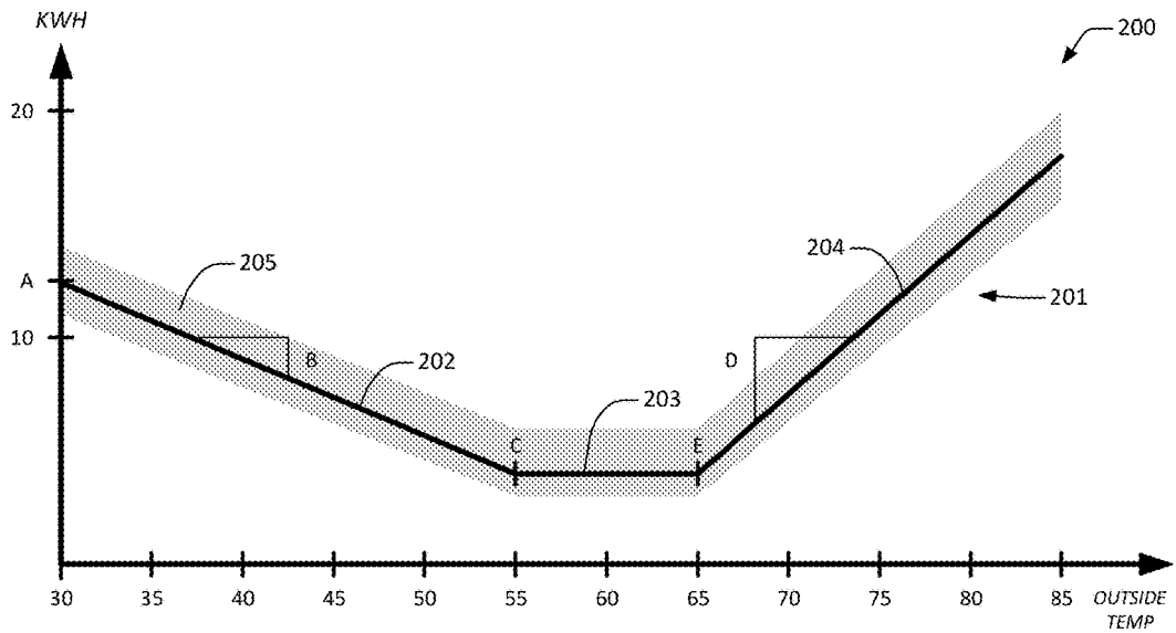
COARSE-GRAINED 5-PARAMETER REGRESSION BASELINE MODEL
