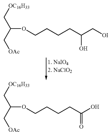
Scheme IX
