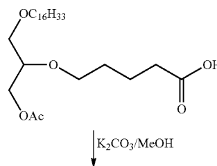
Scheme X
