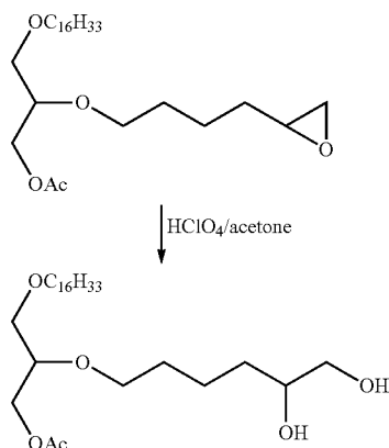
Scheme VIII
