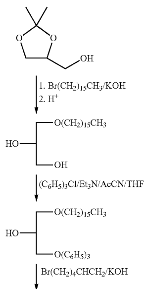
Scheme XV
