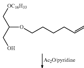
Scheme VII
