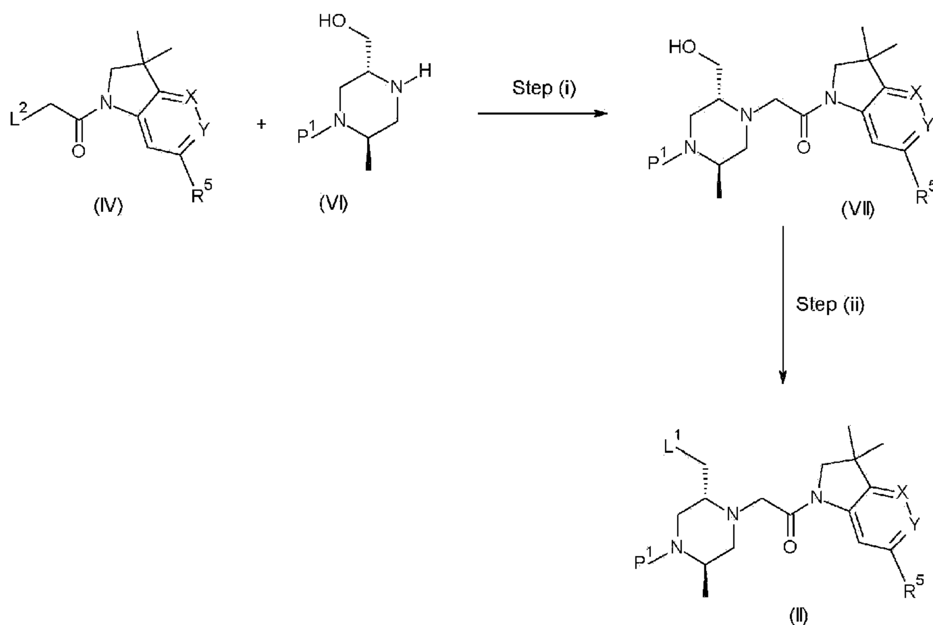
Scheme 1
