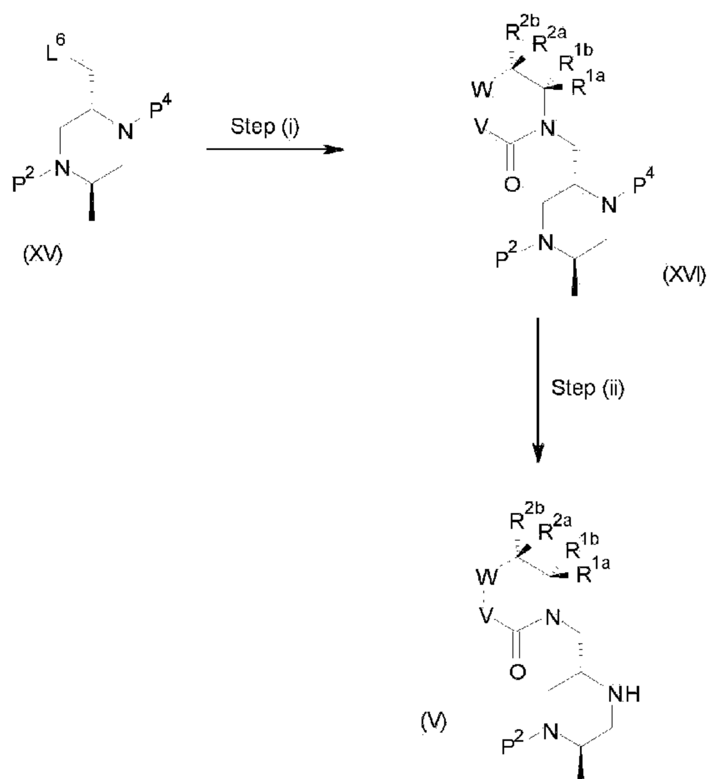
Scheme 3
