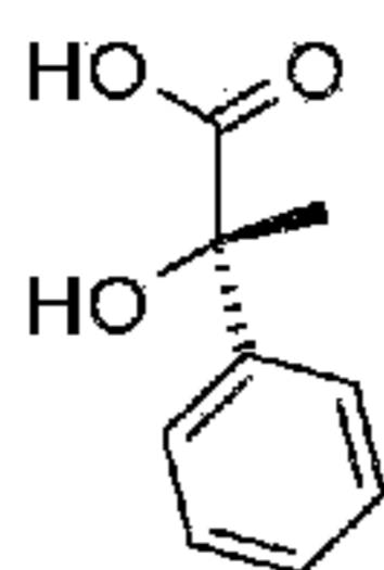
(S)-(+)-2-hydroxy-2-phenylpropionic acid
