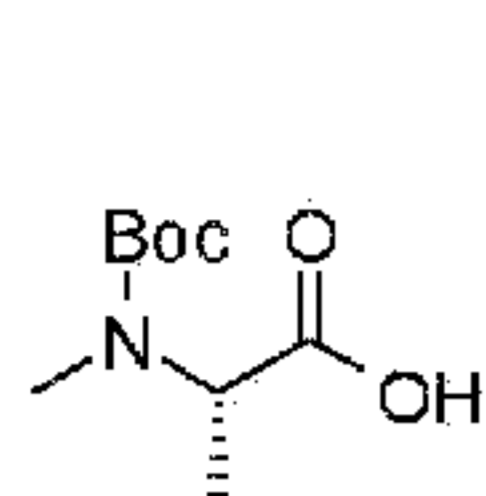
Boc-N-Methyl alanine
