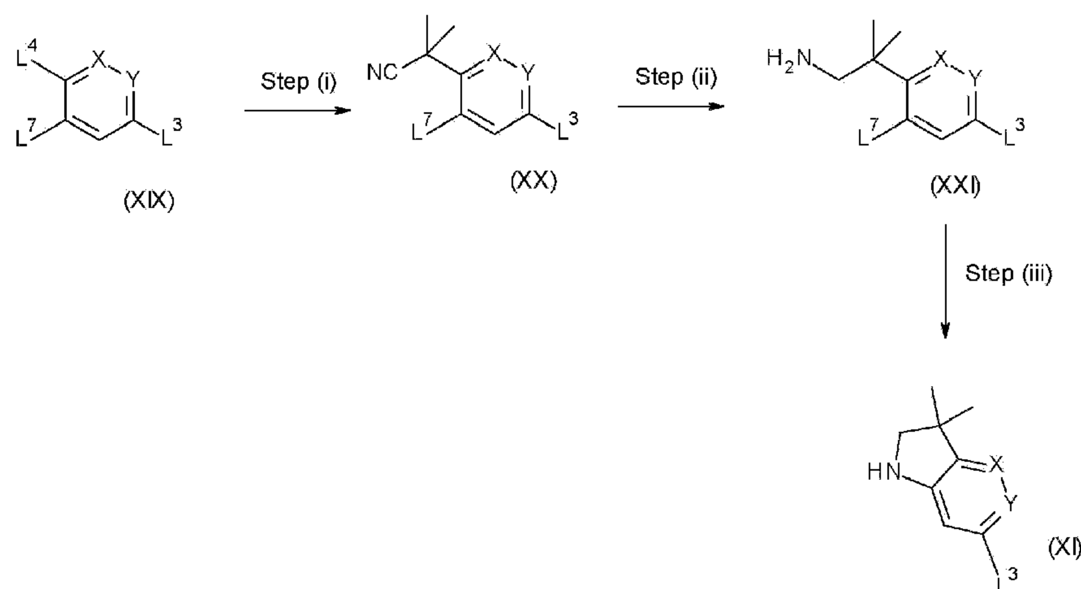
Scheme 4
