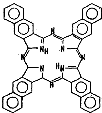
NAPHTHALOCYANINE
