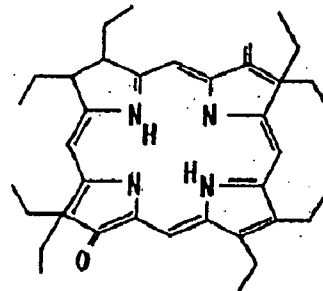
OCTAETHYLDIOXOBACTERIOCHLORIN
