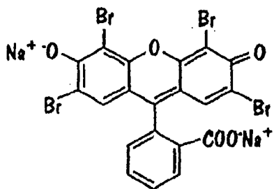
EROSIN Y [FORMULA C]
