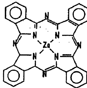
ZINC PHTHALOCYANINE
