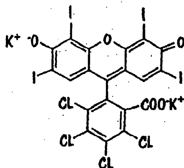
ROSE BENGAL [FORMULA B]
