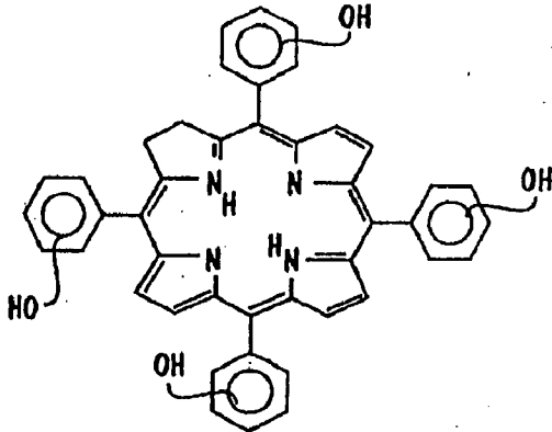
MESO-TETRA (HYDROXYPHENYL) CHLORIN
