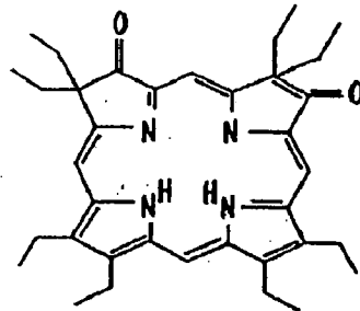
OCTAETHYLDIOXOBACTERIOCHLORIN
