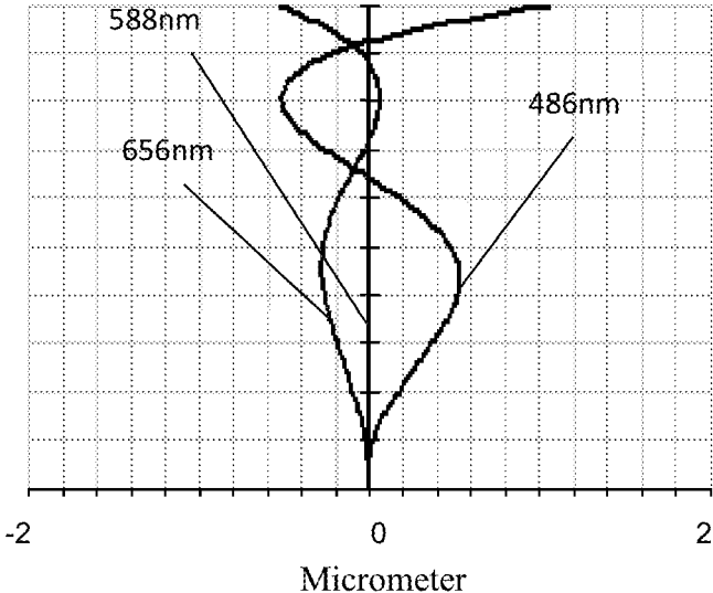
Magnification chromatism
