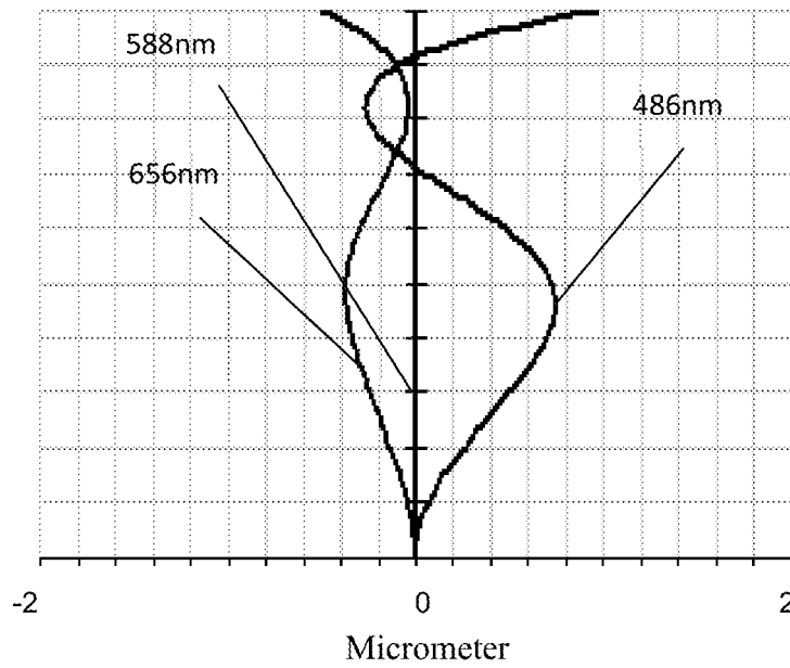
Magnification chromatism
