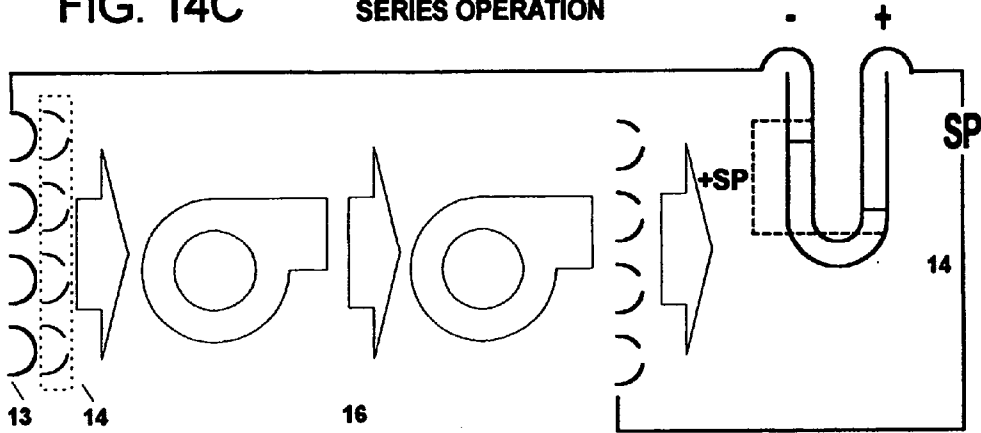
FIG. 14C SERIES OPERATION
