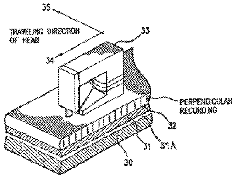
Figure 3. Perspective View of a Magnetic Head and a Magnetic Disk.
