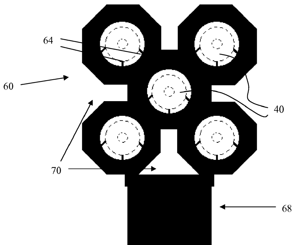
Fig. 6 Another Embodiment of a Substrate Holder
