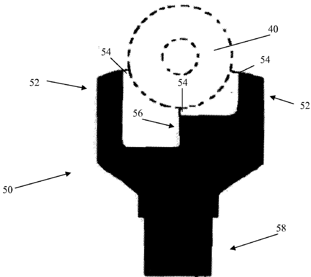
Figure 4. Substrate holder
