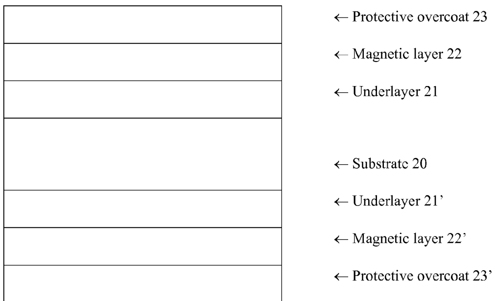
Figure 2. Schematic Representation of the Film Structure in Accordance With a Magnetic Recording Medium.
