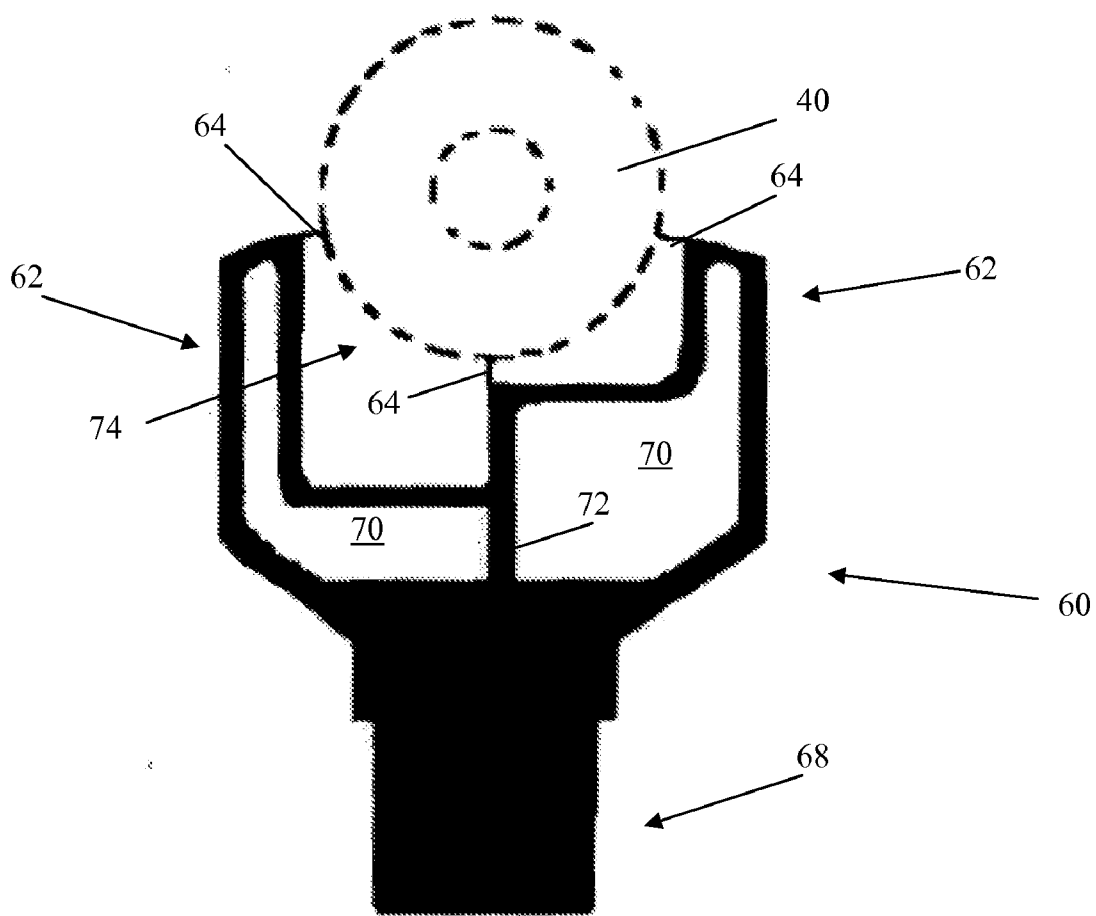
Figure 5. Embodiment of a Substrate holder.
