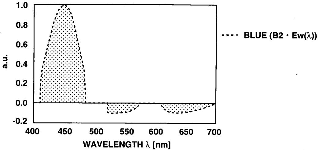
SPECTRAL PRODUCT OF: SPECTRAL SENSITIVITY OF B SIGNAL OF SECOND CCD; AND SPECTRAL PRODUCT E_w(\lambda) INCLUDING BAND-LIMITING FILTER
