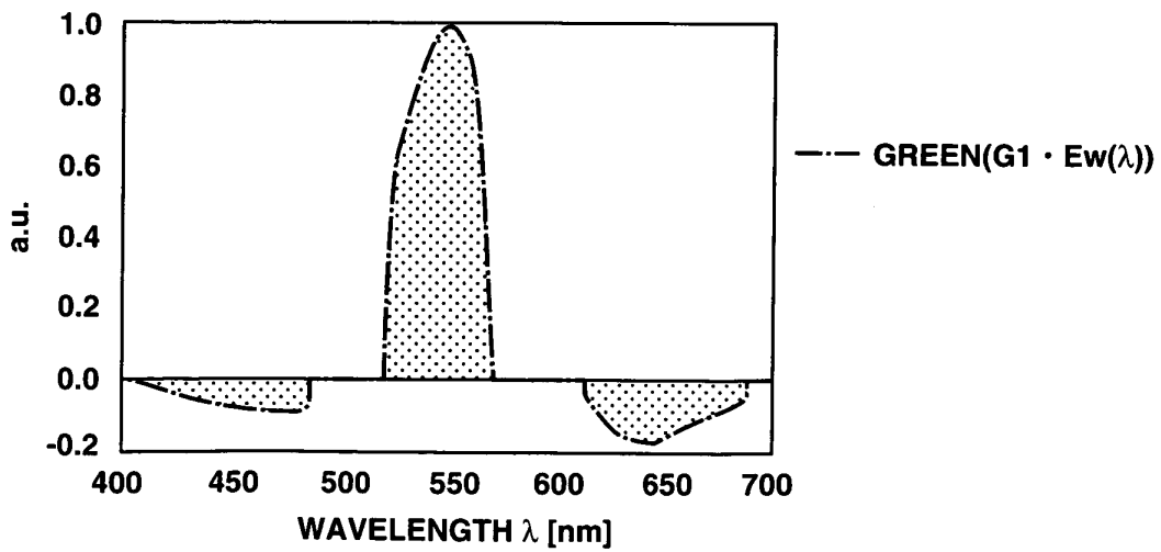
SPECTRAL PRODUCT OF: SPECTRAL SENSITIVITY OF G SIGNAL OF FIRST CCD; AND SPECTRAL PRODUCT E_w(\lambda) INCLUDING BAND-LIMITING FILTER
