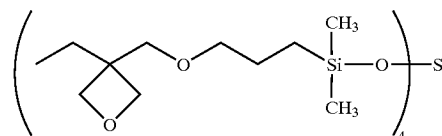
Exemplified Compound 3
