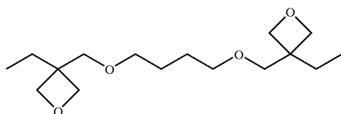
Exemplified Compound 6
