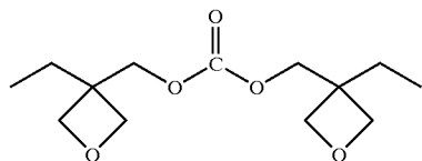
Exemplified Compound 2
