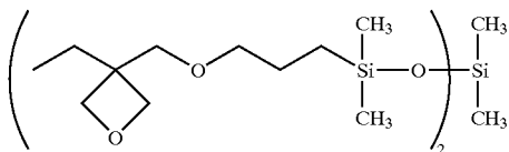
Exemplified Compound 2
