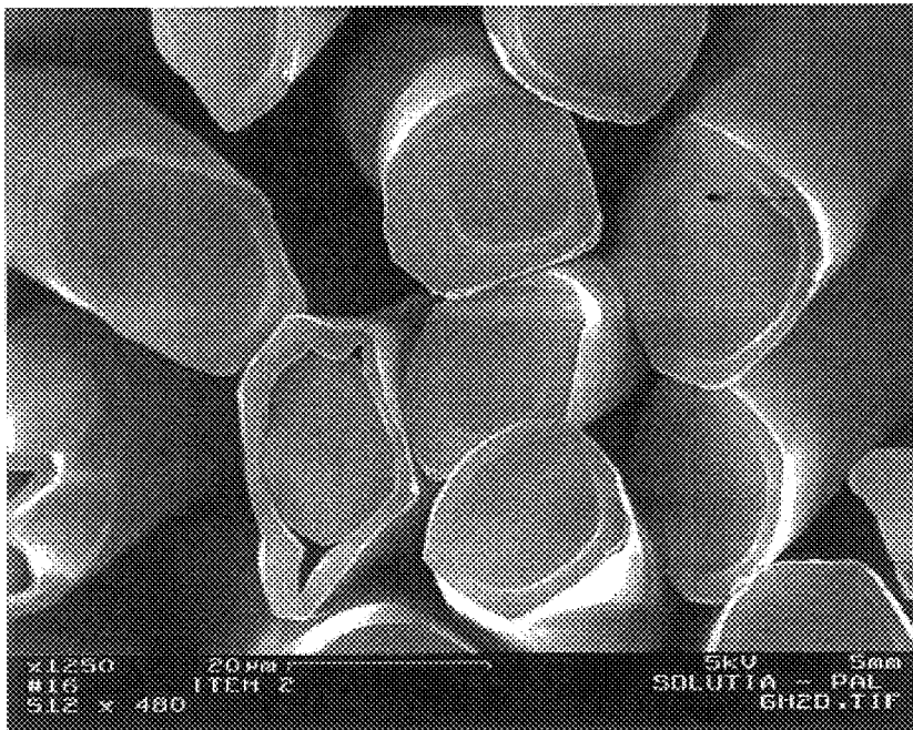
Figure 2 Staple, Drawn Fiber (magnification: x 1250)
