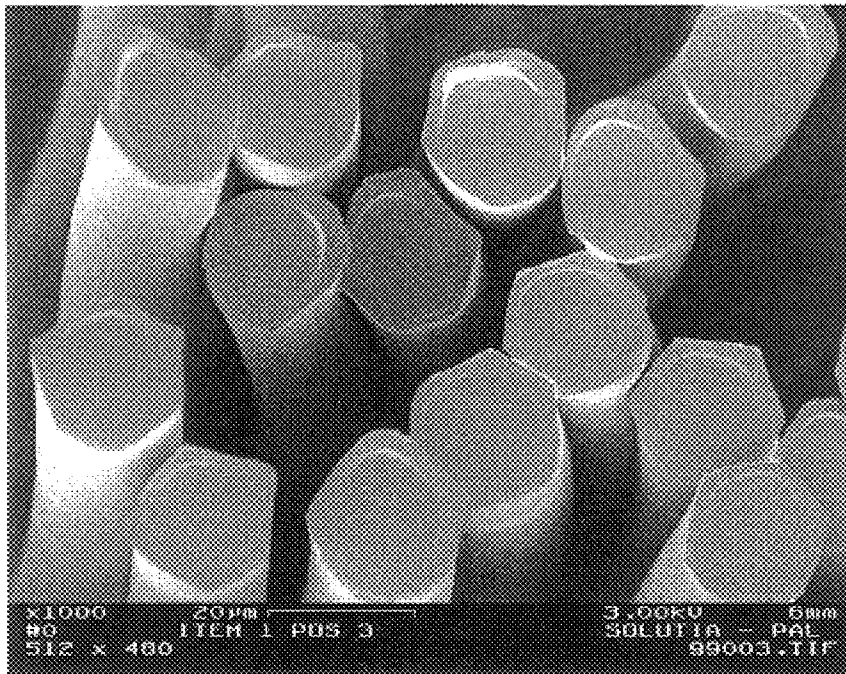
Figure 3 Drawn Yarn, 2-Step (magnification: x 1000)
