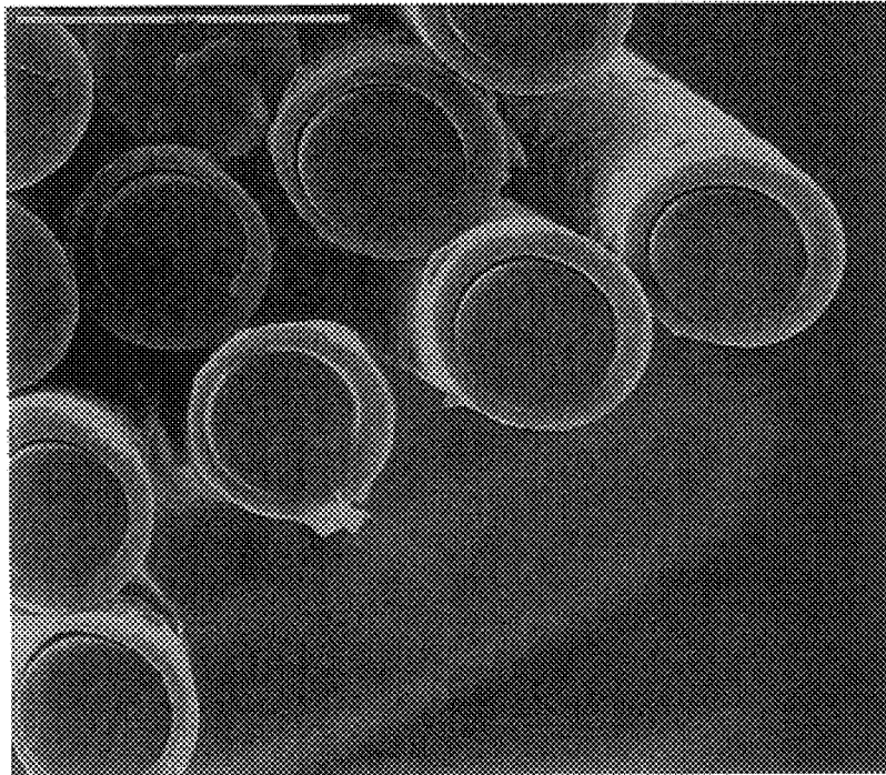
Figure 1 Typical Spun Fiber Cross-Section (magnification: x 1000)
