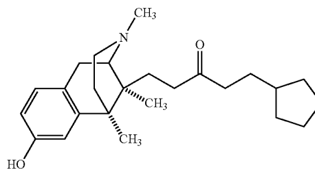
WIN 44,441
