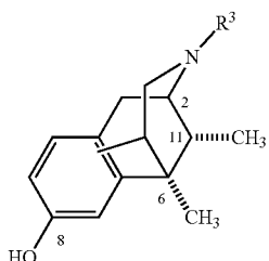
Chart 1. Opioid Receptor Ligands Benzomorphanans (a.k.a. 2,6-Methano-3-benzazocines)
