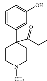
Ketobemidone Registry Number 469-79-4
