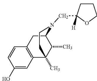
MR2034-“Merz” core structure (opt. active)
