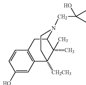
Bremazocine
