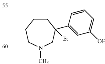
Meptazinol Registry Number 59263-76-2
