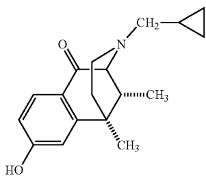
Ketocyclazocine
