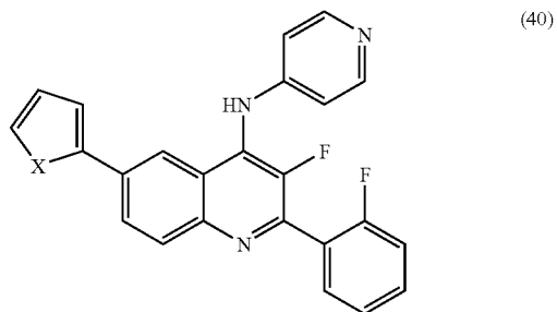
[3-Fluoro-2-(2-fluoro-phenyl)-6-furan-2-yl-quinolin-4-yl]-pyridin-4-yl-amine
