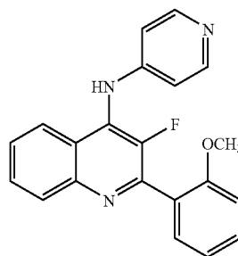
(34) [3-Fluoro-2-(2-methoxy-phenyl)-quinolin-4-yl]-pyridin-4-yl-amine
