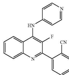
2-[3-Fluoro-4-(pyridin-4-ylamino)-quinolin-2-yl]-benzonitrile
