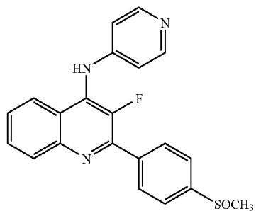
[3-Fluoro-2-(4-methanesulfinyl-phenyl)-quinolin-4-yl]-pyridin-4-yl-amine
