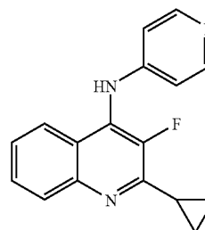
(2-Cyclopropyl-3-fluoro-quinolin-4-yl)-pyridin-4-yl-amine
