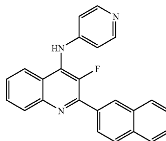
(3-Fluoro-2-naphthalen-2-yl-quinolin-4-yl)-pyridin-4-yl-amine
