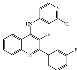
(2-Chloro-pyridin-4-yl)-[3-fluoro-2-(3-fluoro-phenyl)-quinolin-4-yl]-amine
