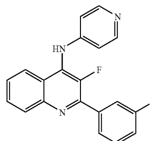
[3-Fluoro-2-(3-fluoro-phenyl)-quinolin-4-yl]-pyridin-4-yl-amine
