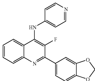
(29) (2-Benzo[1,3]dioxol-5-yl-3-fluoro-quinolin-4-yl)-pyridin-4-yl-amine
