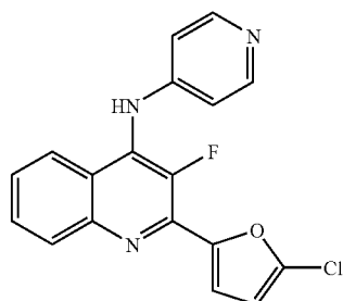
[2-(5-Chloro-furan-2-yl)-3-fluoro-quinolin-4-yl]-pyridin-4-yl-amine
