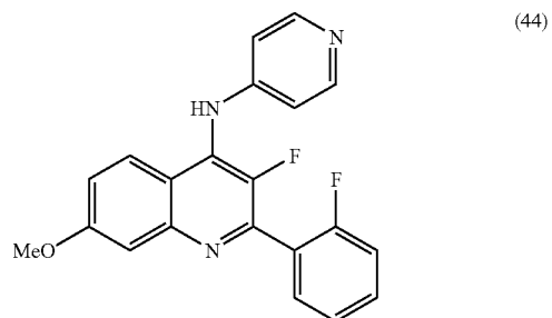
[3-Fluoro-2-(2-fluoro-phenyl)-7-methoxy-quinolin-4-yl]-pyridin-4-yl-amine
