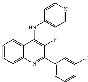
[3-Fluoro-2-(3-fluoro-phenyl)- quinolin-4-yl]-pyridin-4-yl-amine
