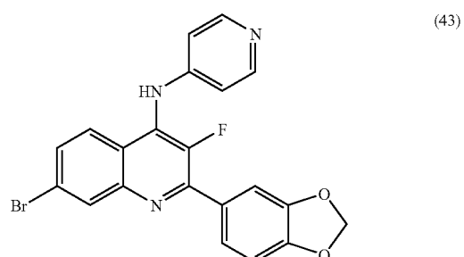
(2-Benzo[1,3]dioxol-5-yl-7-bromo-3-fluoro-quinolin-4-yl)-pyridin-4-yl-amine
