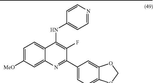
(2-Benzo[1,3]dioxol-5-yl-3-fluoro-7-methoxy-quinolin-4-yl)-pyridin-4-yl-amine
