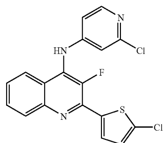
(2-Chloro-pyridin-4-yl)-[2-(5-chloro-thiophen-2-yl)-3-fluoro-quinolin-4-yl]-amine
