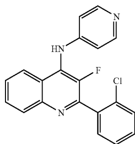
(32) [2-(2-Chloro-phenyl)-3-fluoro-quinolin-4-yl]-pyridin-4-yl-amine
