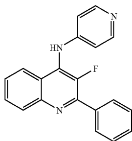
(3-Fluoro-2-phenyl-quinolin-4-yl)-pyridin-4-yl-amine
