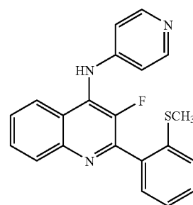
[3-Fluoro-2-(2-methylsulfanylphenyl)-quinolin-4-yl]-pyridin-4-yl-amine
