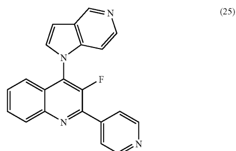
3-Fluoro-2-pyridin-4-yl-4-pyrrolo[3,2-c]pyridin-1-yl-quinoline
