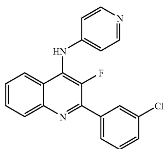
[2-(3-Chloro-phenyl)-3-fluoro- quinolin-4-yl]-pyridin-4-yl-amine
