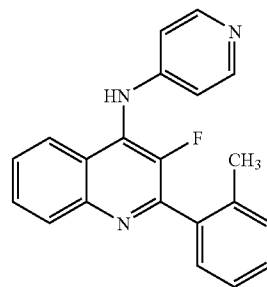
(33) (3-Fluoro-2-o-tolyl-quinolin-4-yl)-pyridin-4-yl-amine
