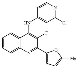
(2-Chloro-pyridin-4-yl)-[3-(fluoro-2-(5-methyl-furan-2-yl)-quinolin-4-yl)]-amine
