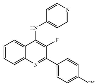
4-[3-Fluoro-4-(pyridin-4-ylamino)-quinolin-2-yl]-benzotrile
