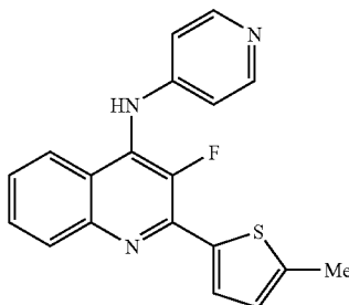
[3-Fluoro-2-(5-methyl-thiophen-2-yl)-quinolin-4-yl]-pyridin-4-yl-amine
