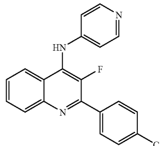
[2-(4-Chloro-phenyl)-3-fluoro- quinolin-4-yl]-pyridin-4-yl-amine
