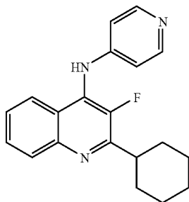
(2-Cyclohexyl-3-fluoro-quinolin-4-yl)-pyridin-4-yl-amine
