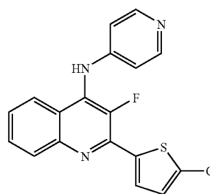
[2-(5-Chloro-thiophen-2-yl)-3-fluoro-quinolin-4-yl]-pyridin-4-yl-amine
