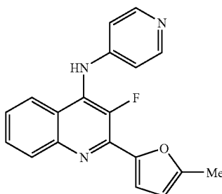
[3-Fluoro-2-(5-methyl-furan-2-yl)-quinolin-4-yl]-pyridin-4-yl-amine
