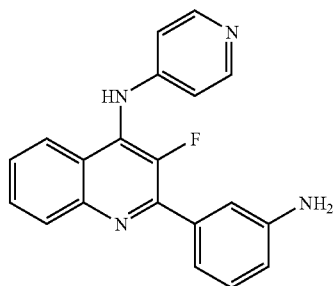
[2-(3-Amino-phenyl)-3-fluoro-quinolin-4-yl]-pyridin-4-yl-amine
