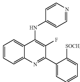
[3-Fluoro-2-(2-methylsulfonylphenyl)-quinolin-4-yl]-pyridin-4-yl-amine
