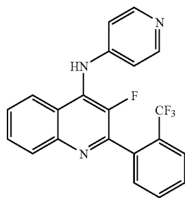
(30) [3-Fluoro-2-(2-trifluoromethyl-phenyl)-quinolin-4-yl]-pyridin-4-yl-amine
