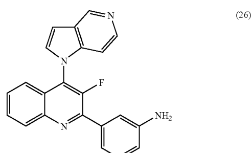
3-(3-Fluoro-4-pyrrolo[3,2c]pyridin-1-yl-quinolin-2-yl)-phenylamine
