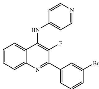
[2-(3-Bromo-phenyl)-3-fluoro-quinolin-4-yl]-pyridin-4-yl-amine
