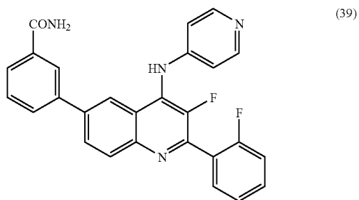
3-[3-Fluoro-2-(2-fluoro-phenyl)-4-(pyridin-4-ylamino)-quinolin-6-yl]-benzamide
