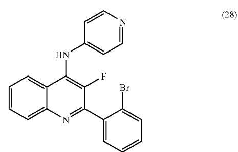
[2-(2-Bromo-phenyl)-3-fluoro-quinolin-4-yl]-pyridin-4-yl-amine
