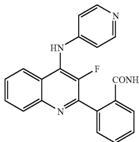
2-[3-Fluoro-4-(pyridin-4-ylamino)-quinolin-2-yl]-benzamide
