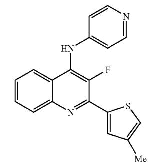
[3-Fluoro-2-(4-methyl-thiophen-2-yl)-quinolin-4-yl]-pyridin-4-yl-amine
