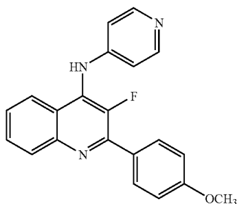
[3-Fluoro-2-(4-methoxy-phenyl)- quinolin-4-yl]-pyridin-4-yl-amine
