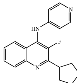
(2-Cyclopentyl-3-fluoro-quinolin-4-yl)-pyridin-4-yl-amine
