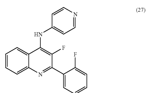
[3-Fluoro-2-(2-fluoro-phenyl)-quinolin-4-yl]-pyridin-4-yl-amine
