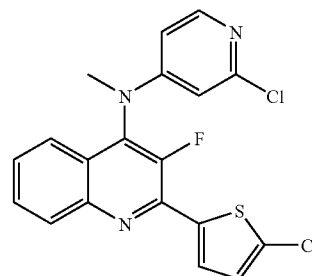
(2-Chloro-pyridin-4-yl)-[2-(5-chloro-thiophen-2-yl)-3-fluoro-quinolin-4-yl]-methyl-amine
