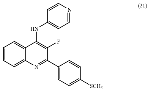
[3-Fluoro-2-(4-methylsulfanyl-phenyl)-quinolin-4-yl]-pyridin-4-yl-amine
