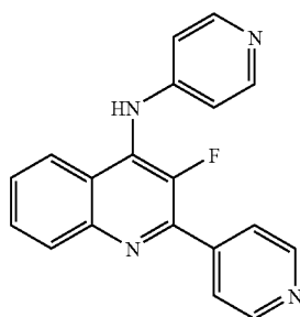
(31) (3-Fluoro-2-pyridin-4-yl-quinolin-4-yl)-pyridin-4-yl-amine
