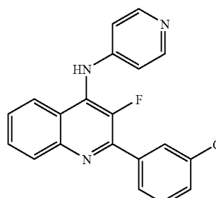
[2-(3-Chloro-phenyl)-3-fluoro-quinolin-4-yl]-pyridin-4-yl-amine
