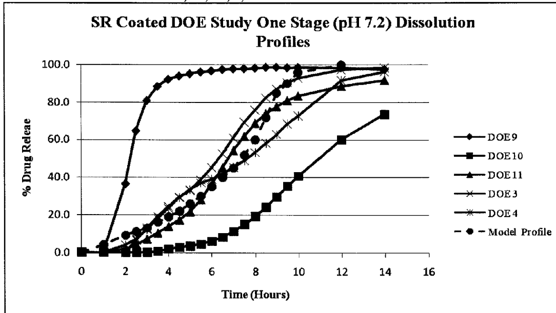
Dissolution Profiles of DOE 9, 10, 11, 3, 4
