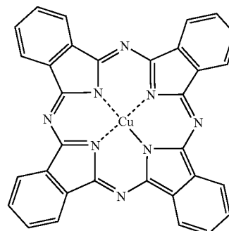
Cu-Phthalocyanine
