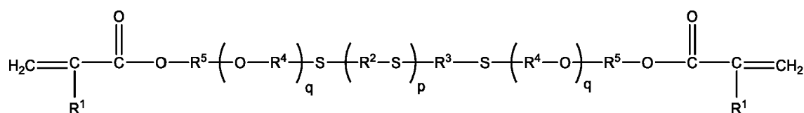
Formula (Ia)
