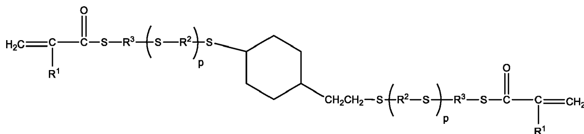
Formula (IIc)
