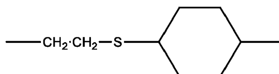
Formula (E)
