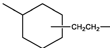
Formula (G-2)
