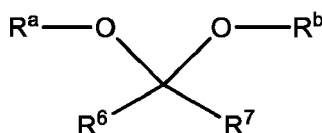
Formula (a-1)
