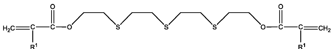
Formula (Ib)
