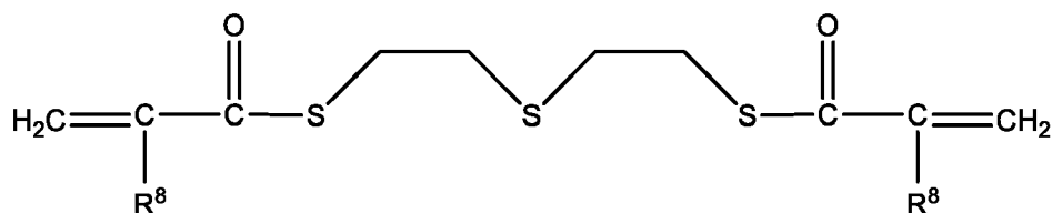
Formula (IIb)
