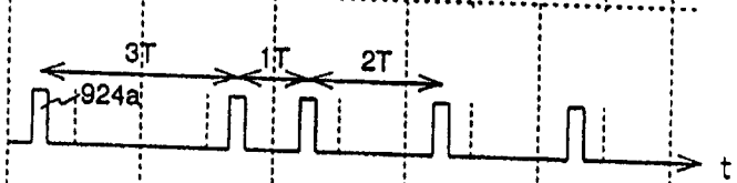
Fig. 3c Recorded Signal
