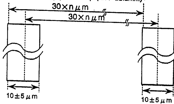
Fig. 5b Slit Dimension Accuracy (Precision) (at r=22.2mm )
