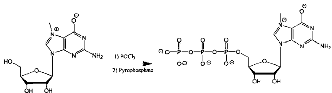
Scheme 5
