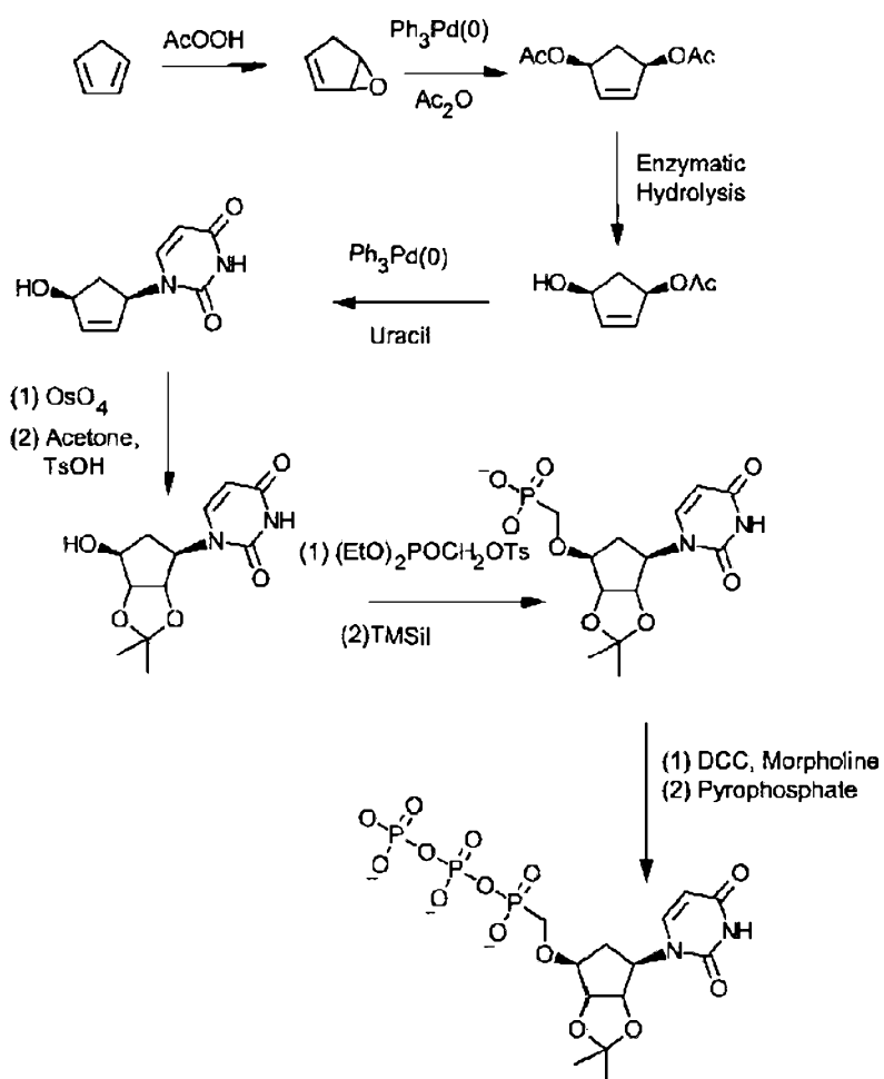
Scheme 9
