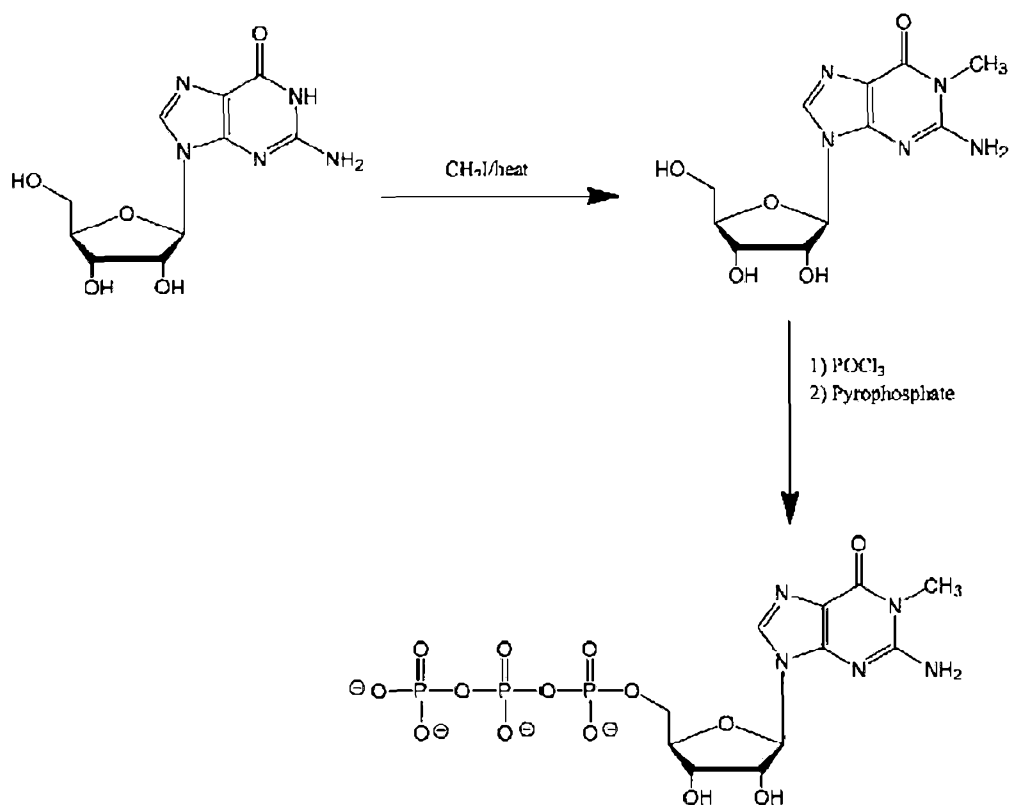
Scheme 4
